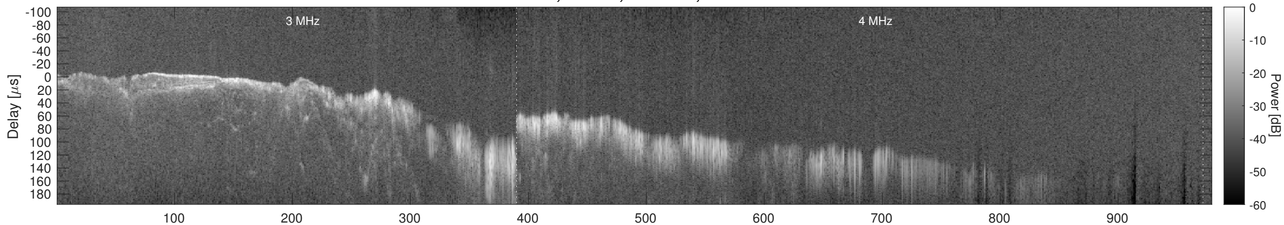
Orbit 12646, Window, Channel 2, Chapman
