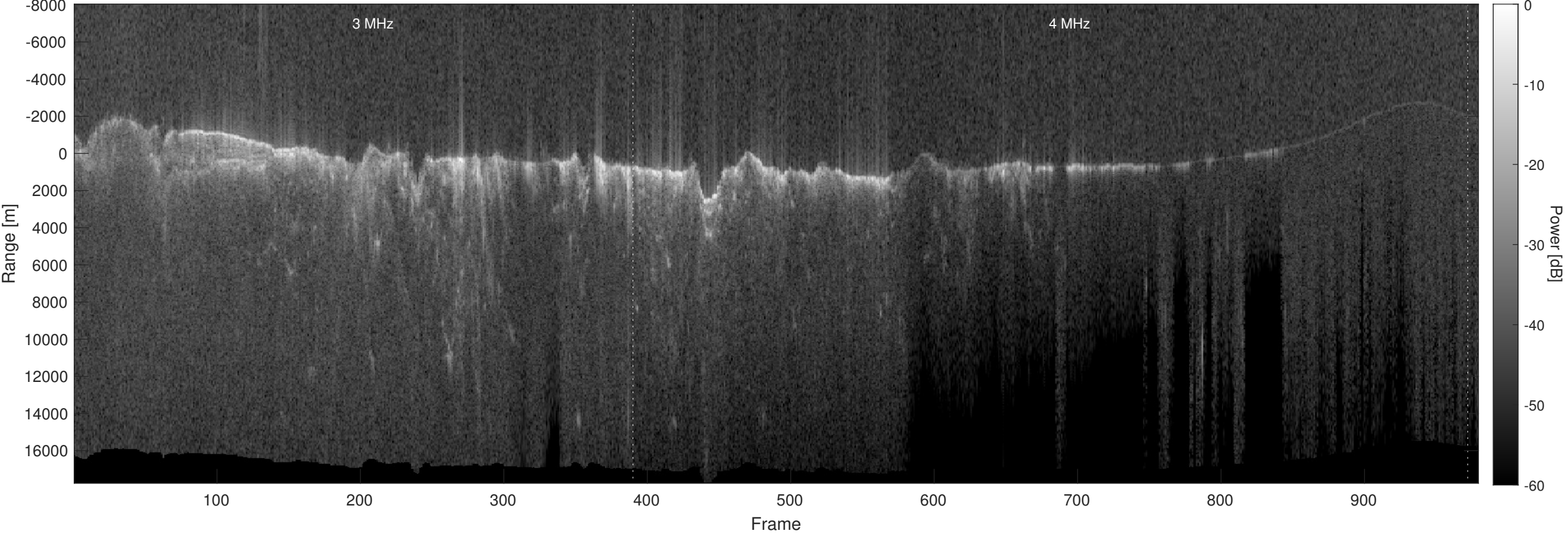
Orbit 12646, Optimized, No Window, Depth-Corrected, Channel 2
