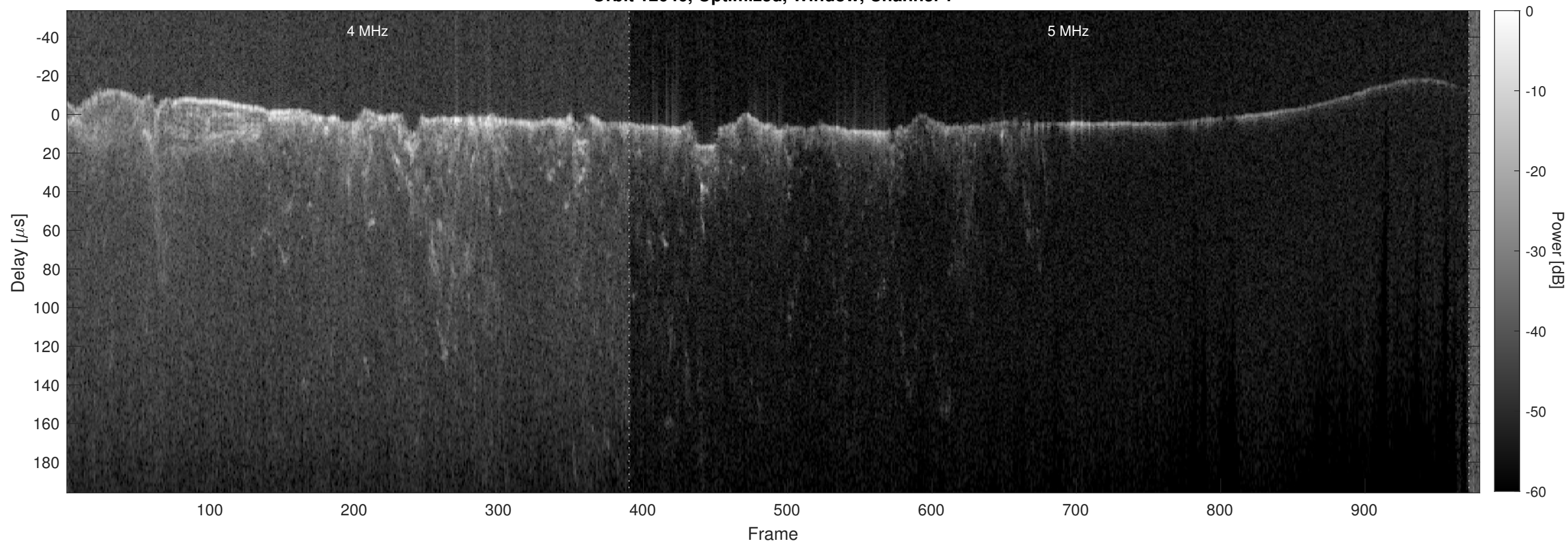
Orbit 12646, Optimized, Window, Channel 2
