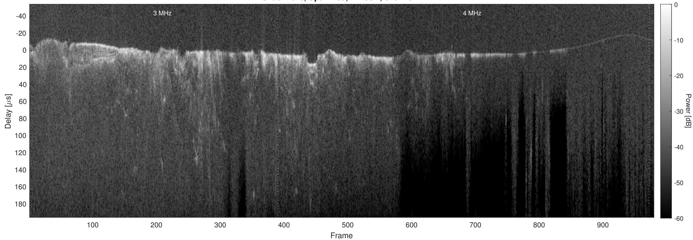
Orbit 12646, Optimized, Window, Channel 2
