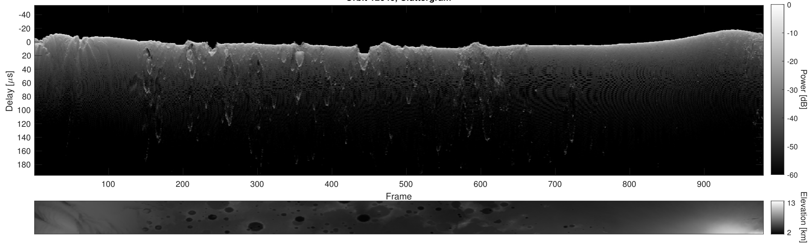
Orbit 12646, Cluttergram
