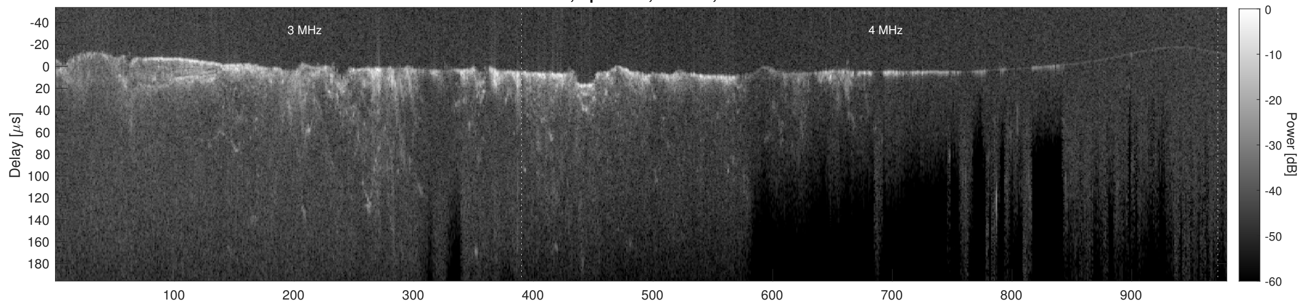
Orbit 12646, Cluttergram
