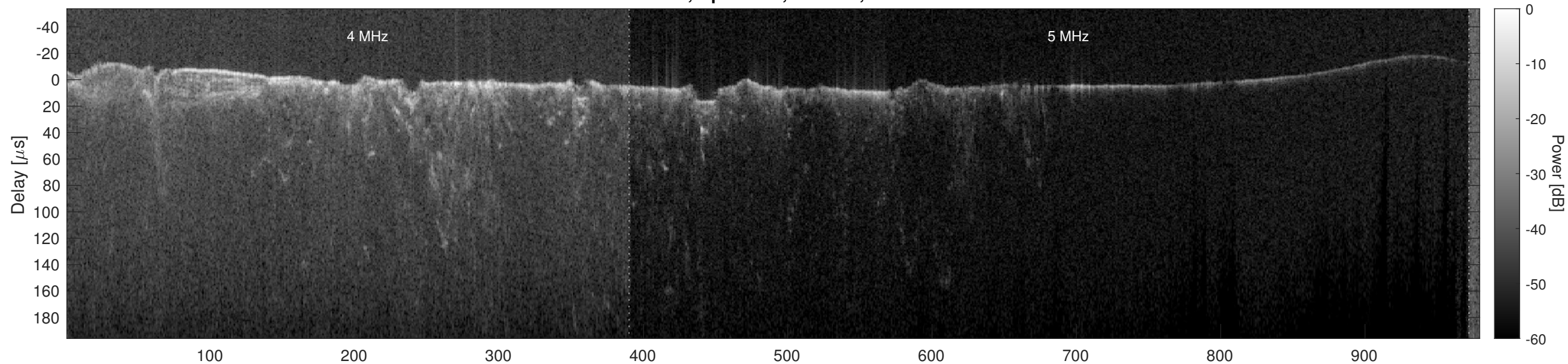
Orbit 12646, Optimized, Window, Channel 2
