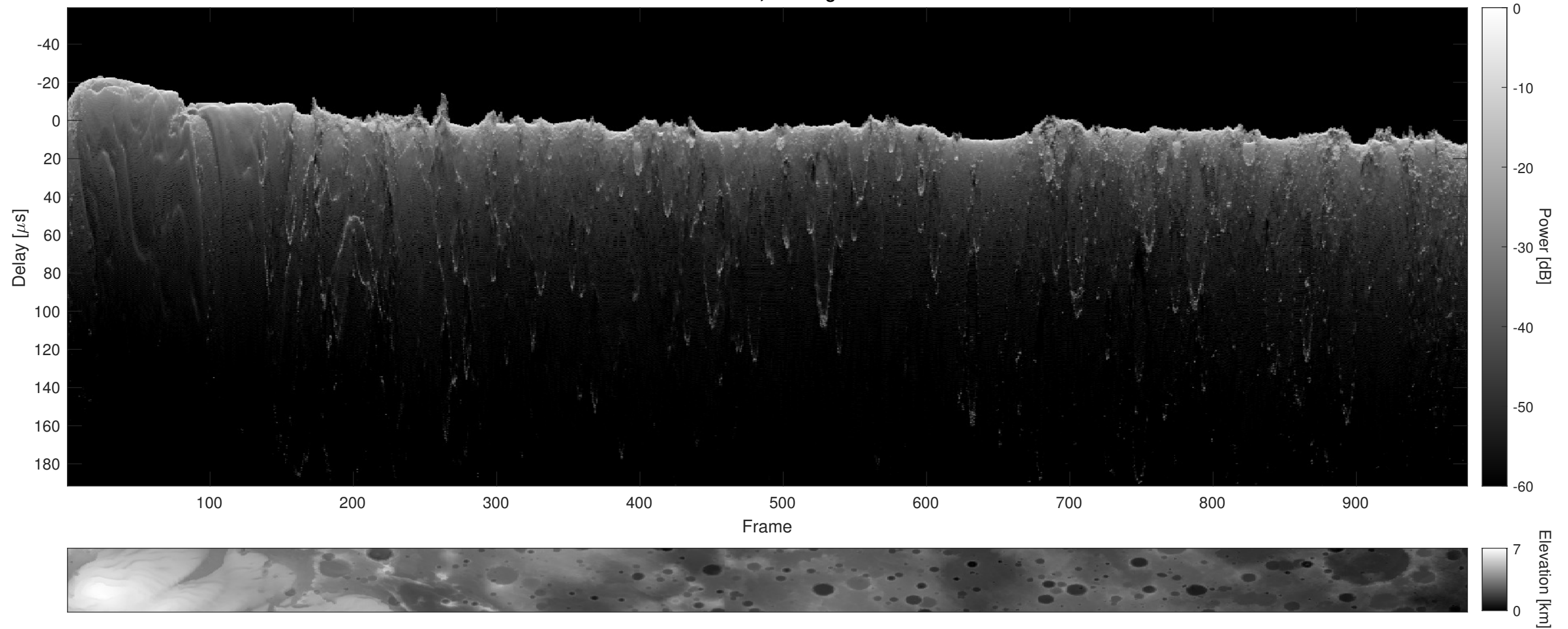
Orbit 12647, Cluttergram
