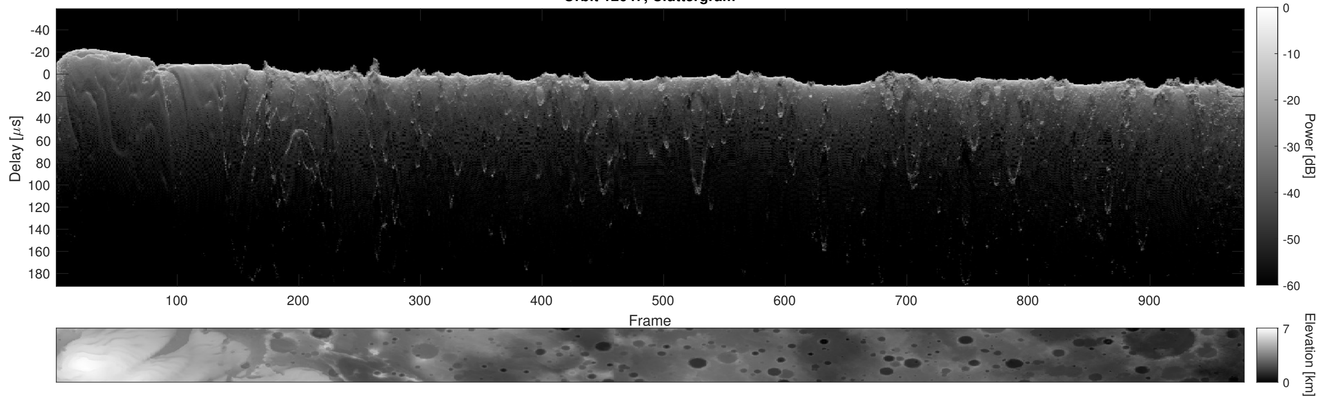
Orbit 12647, Cluttergram
