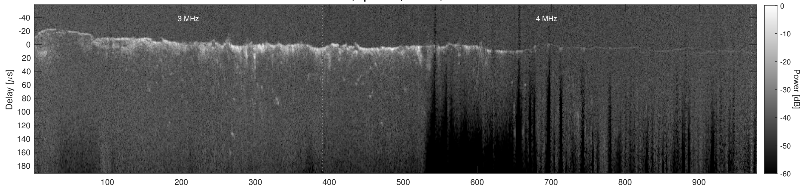
Orbit 12647, Cluttergram
