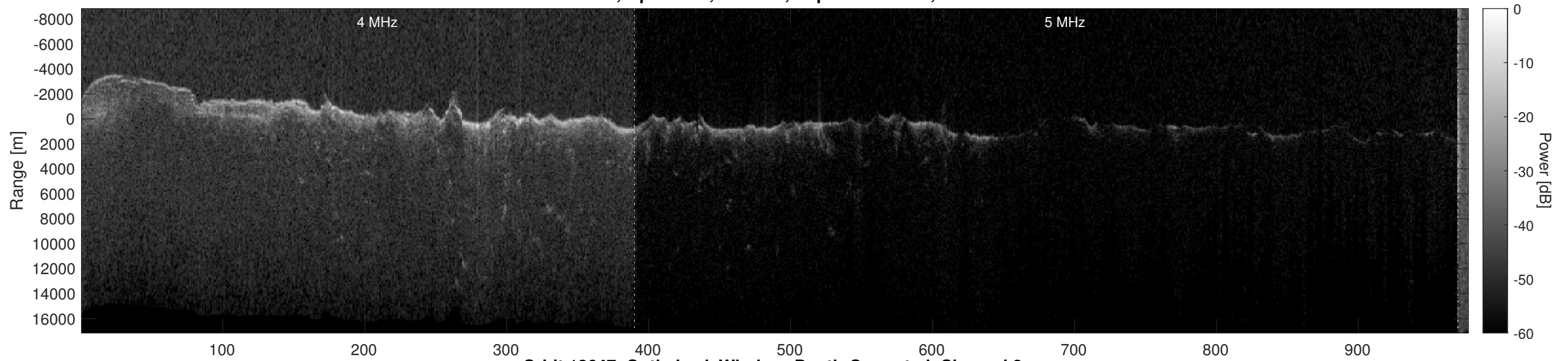
Orbit 12647, Optimized, Window, Depth-Corrected, Channel 2
