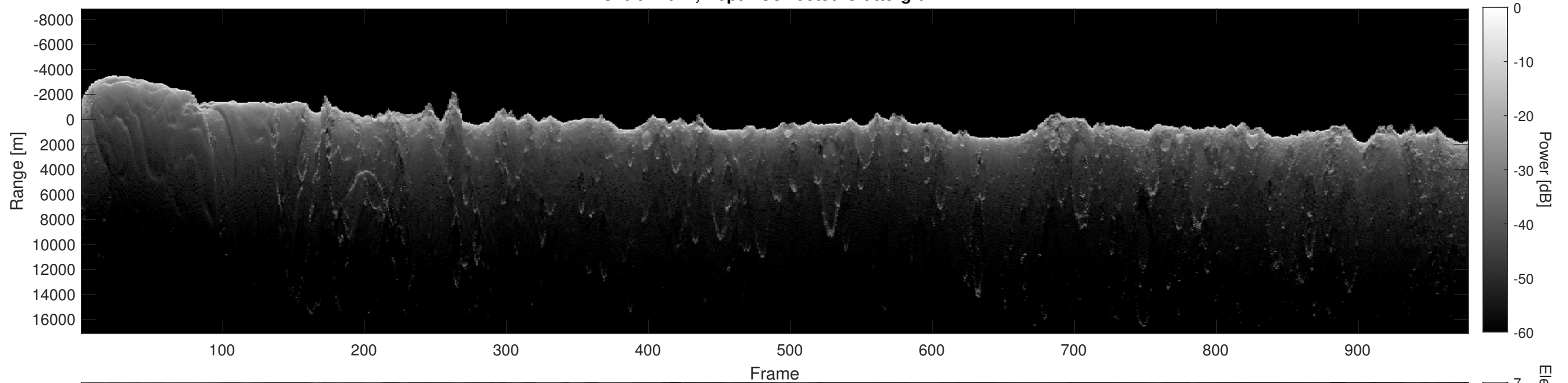
Orbit 12647, Depth-Corrected Cluttergram
