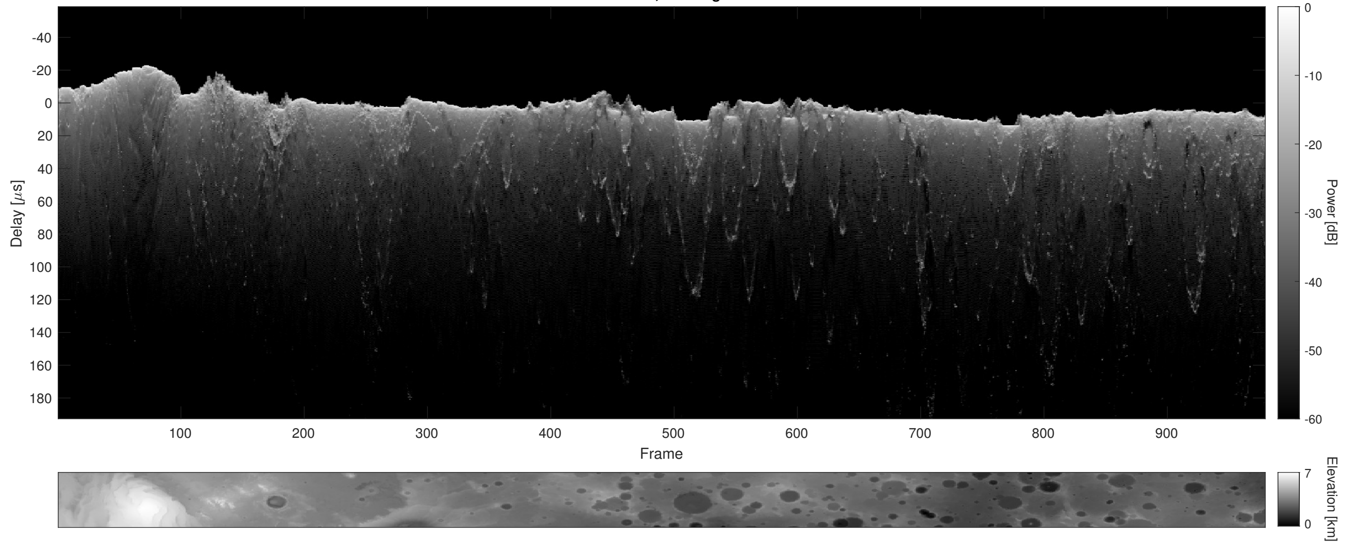
Orbit 12648, Cluttergram
