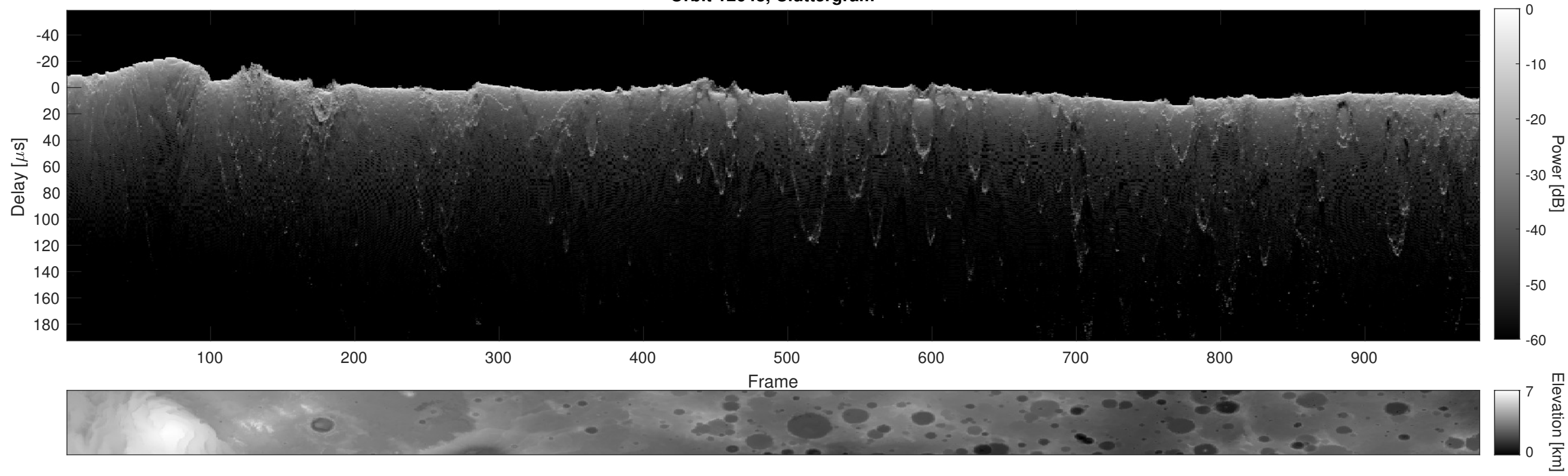
Orbit 12648, Cluttergram
