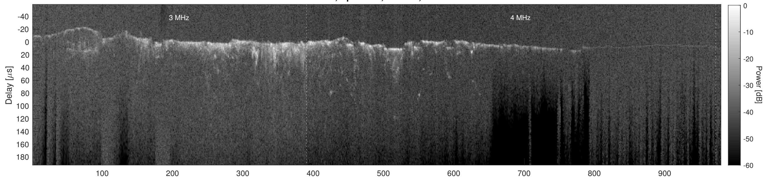
Orbit 12648, Cluttergram
