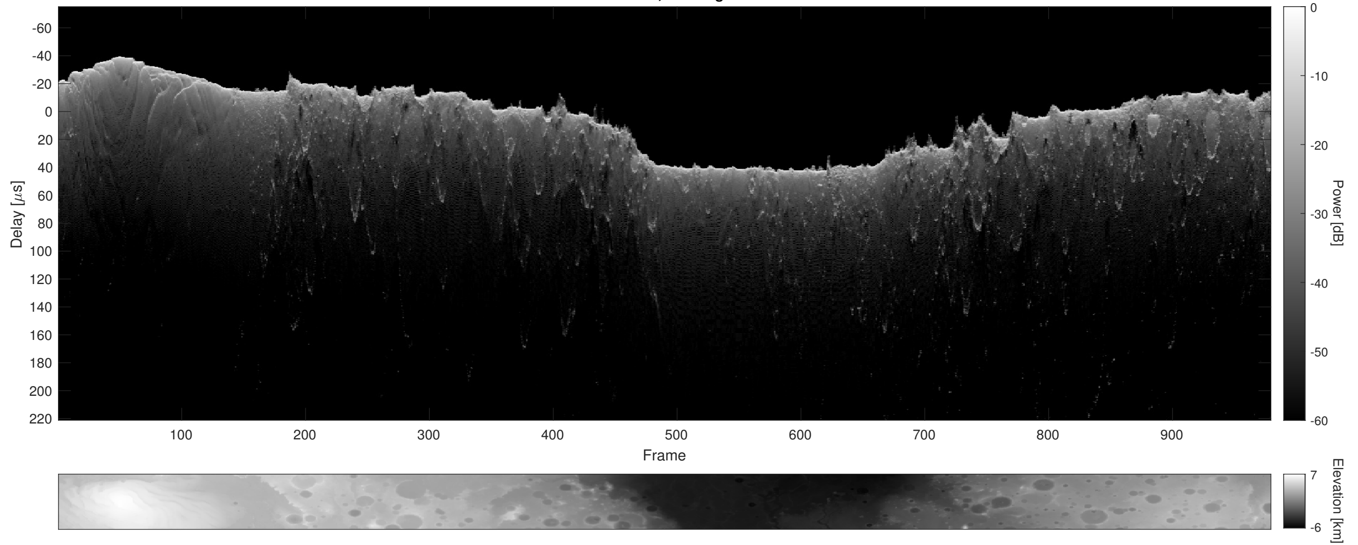
Orbit 12651, Cluttergram
