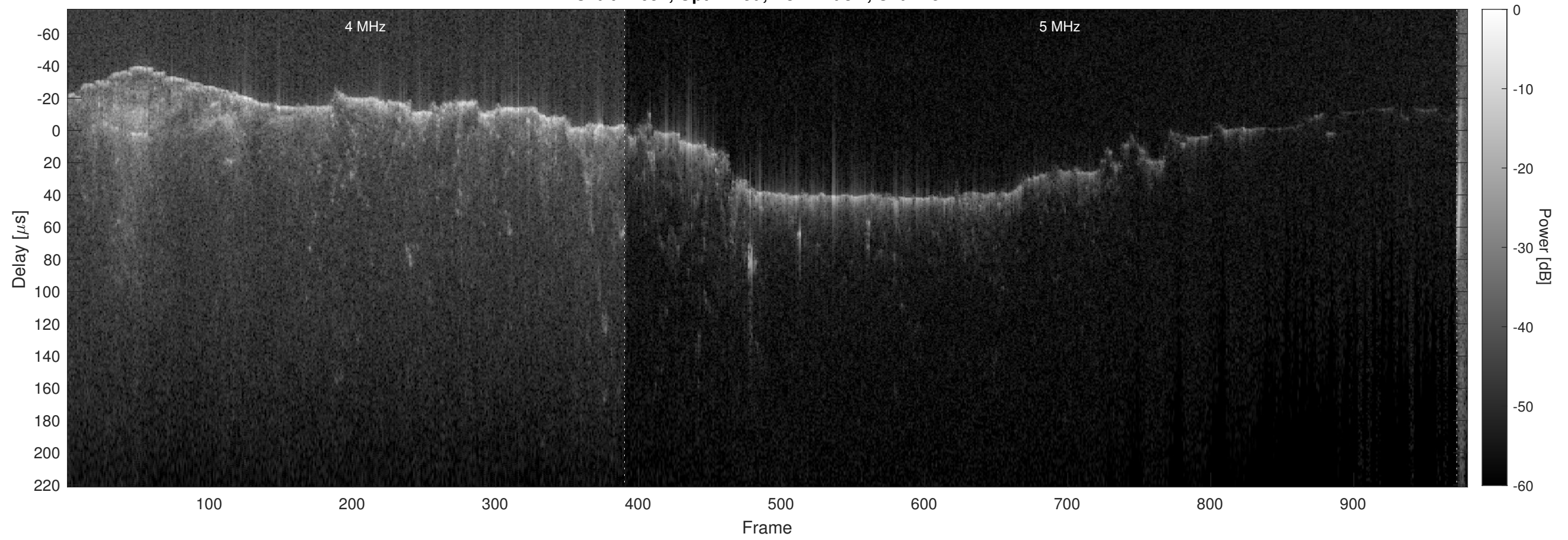
Orbit 12651, Optimized, No Window, Channel 2
