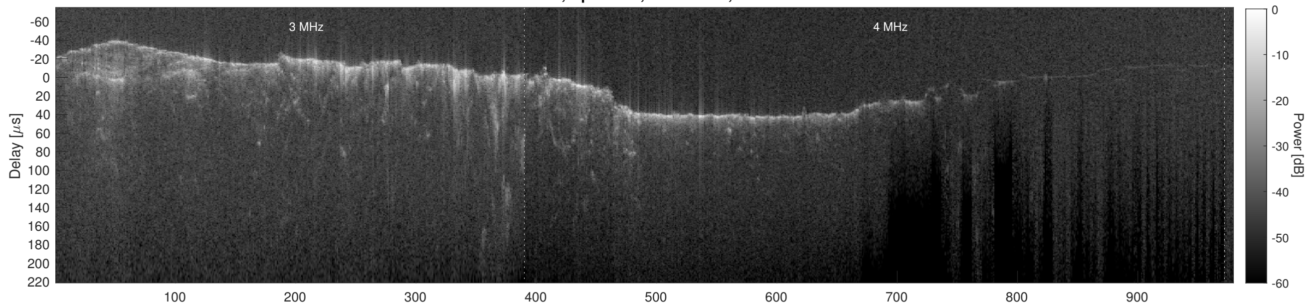
Orbit 12651, Cluttergram
