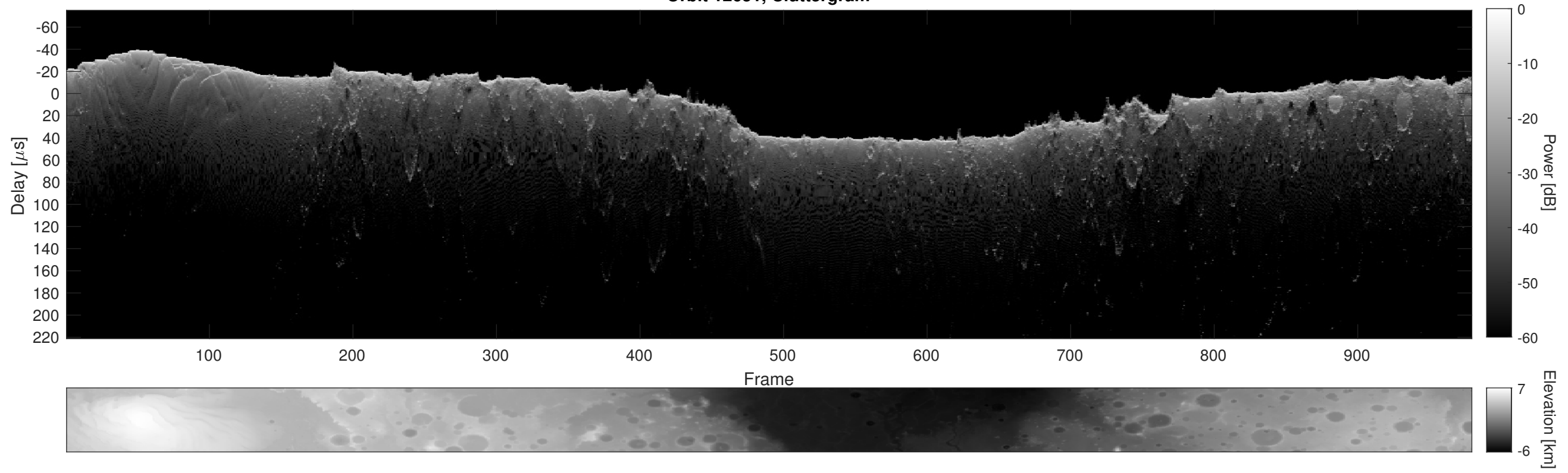
Orbit 12651, Cluttergram
