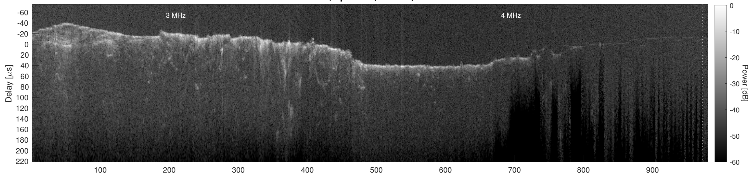
Orbit 12651, Cluttergram
