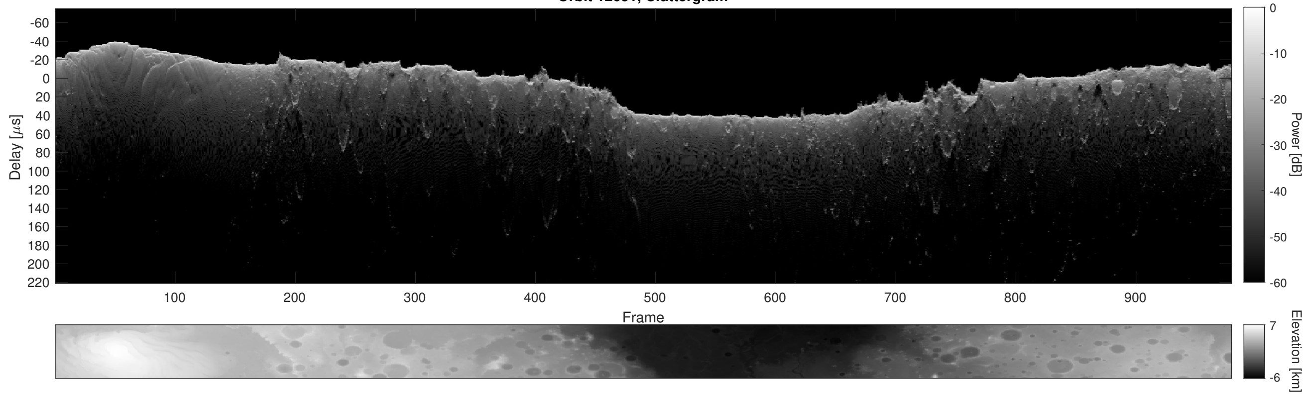
Orbit 12651, Cluttergram
