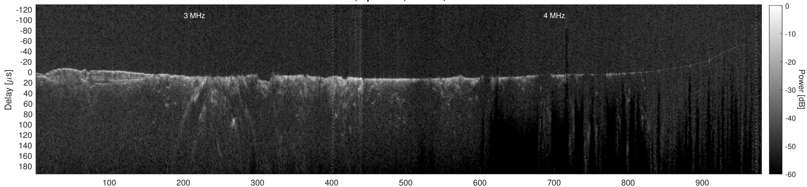
Orbit 12653, Cluttergram
