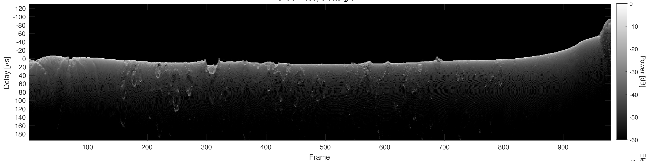
Orbit 12653, Cluttergram
