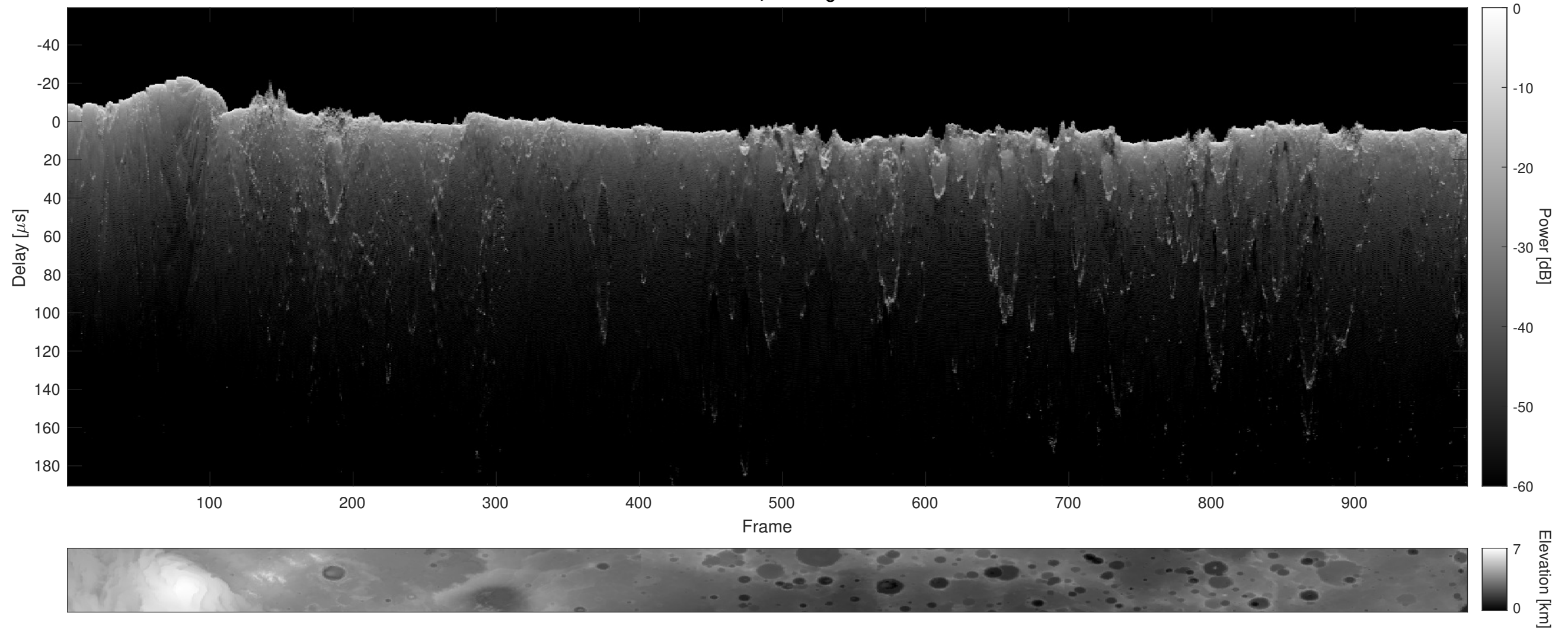
Orbit 12655, Cluttergram
