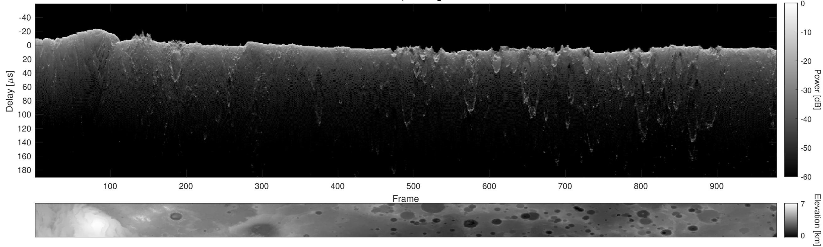
Orbit 12655, Cluttergram
