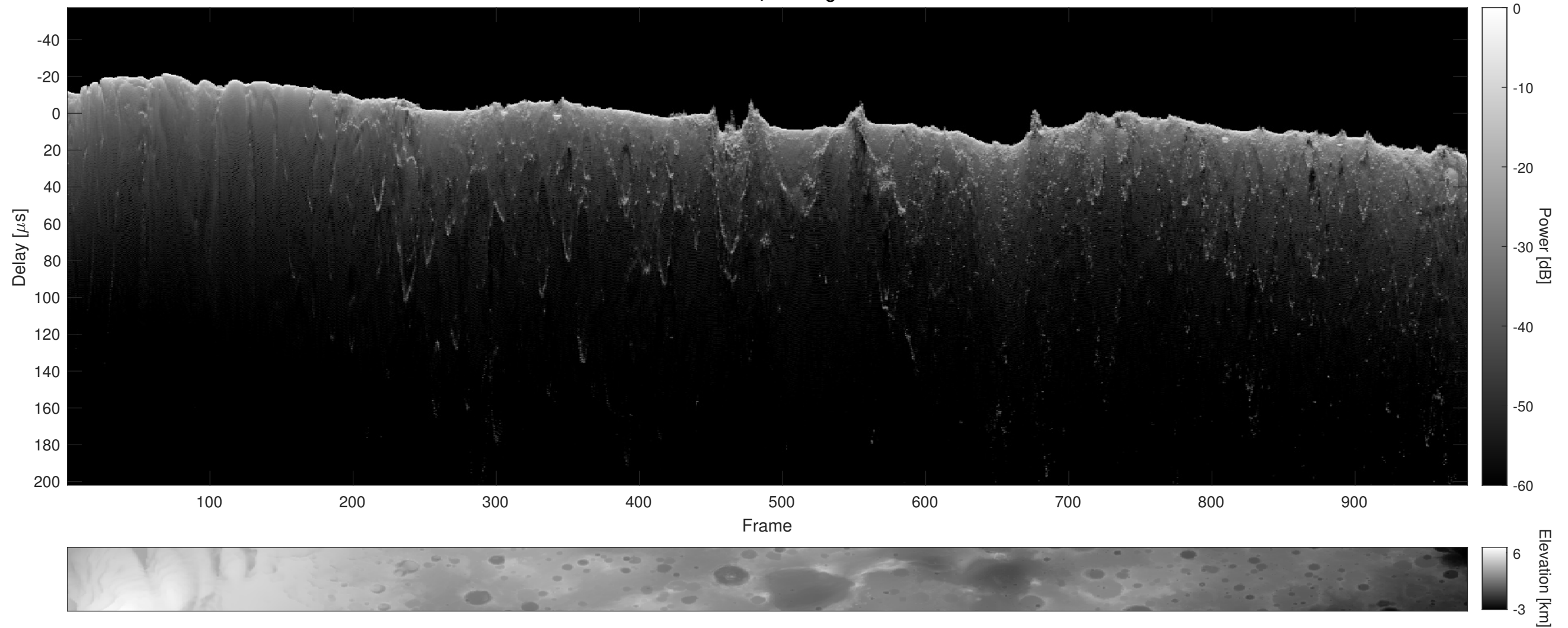
Orbit 12657, Cluttergram
