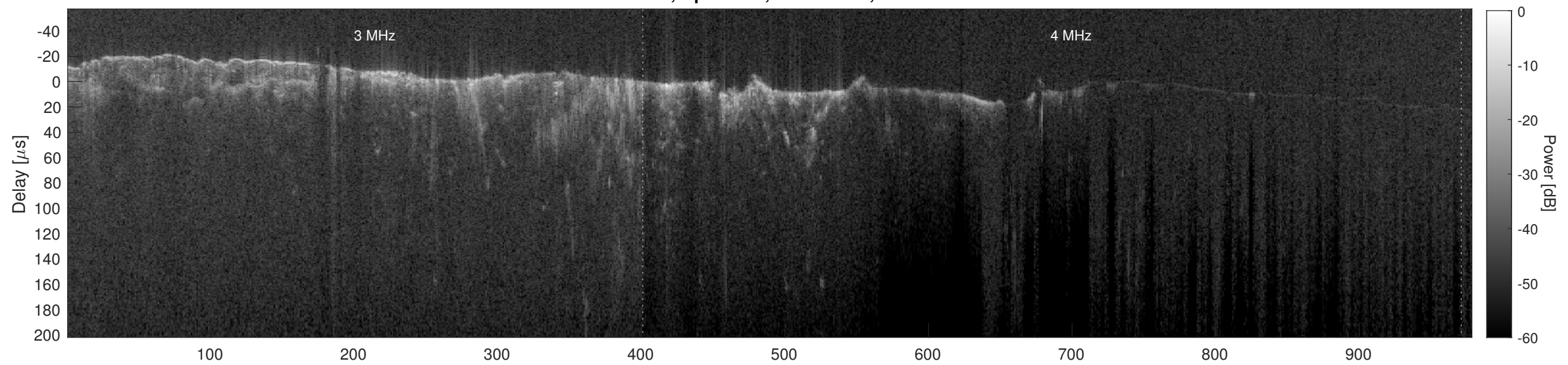
Orbit 12657, Cluttergram
