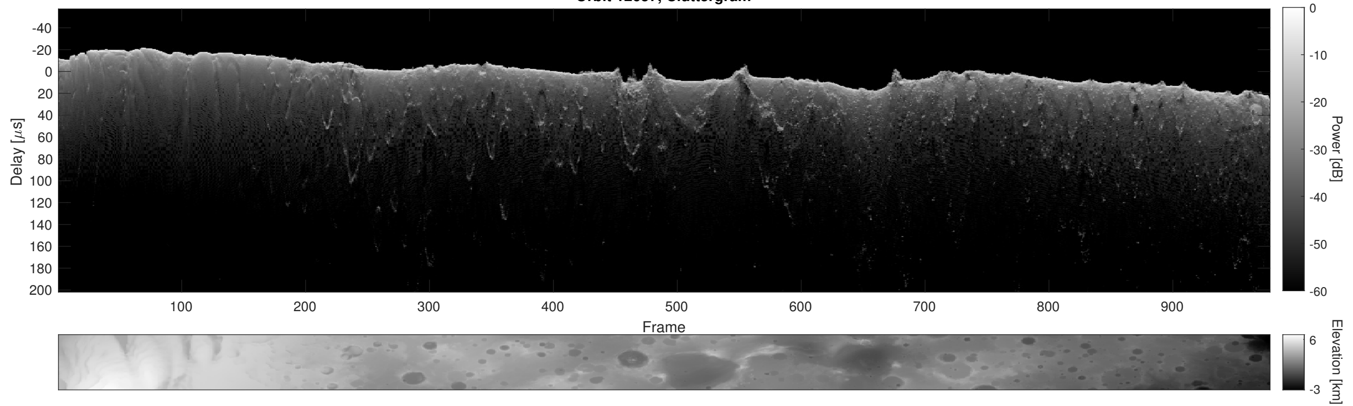
Orbit 12657, Cluttergram
