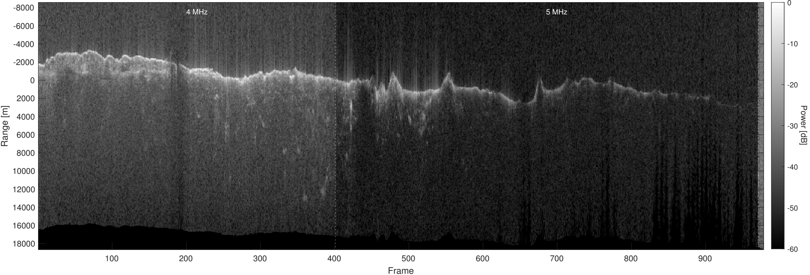
Orbit 12657, Optimized, No Window, Depth-Corrected, Channel 2
