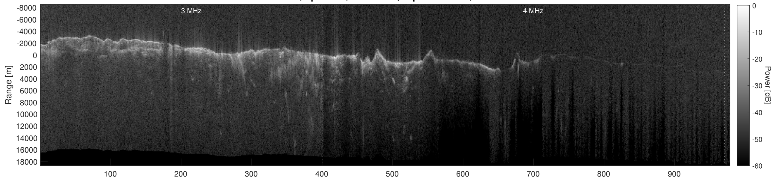
Orbit 12657, Depth-Corrected Cluttergram
