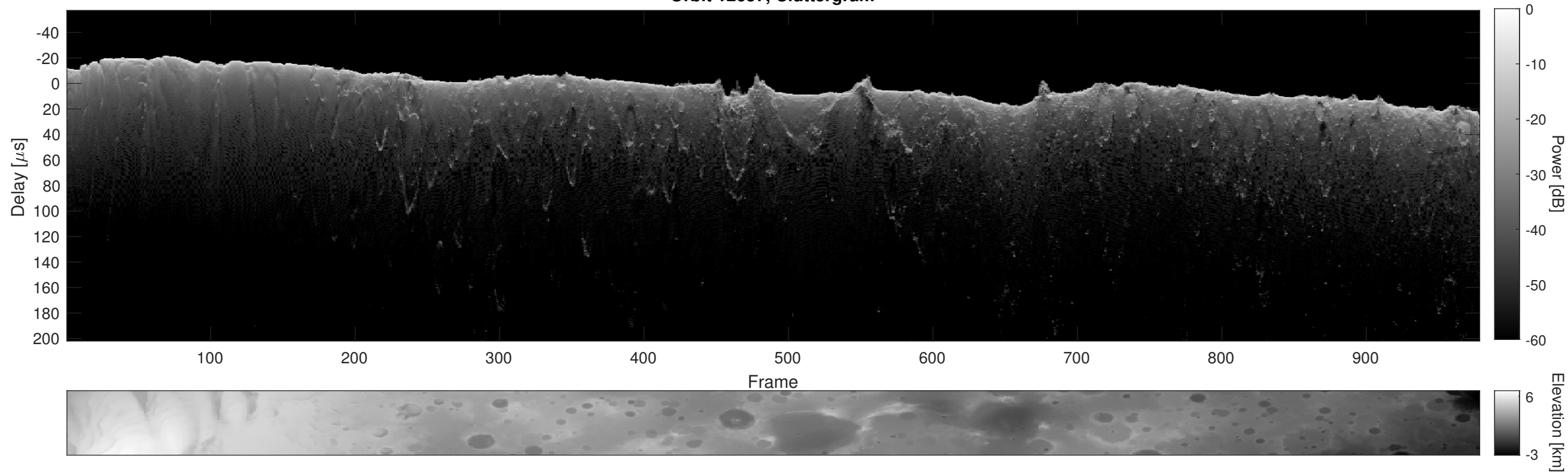
Orbit 12657, Cluttergram
