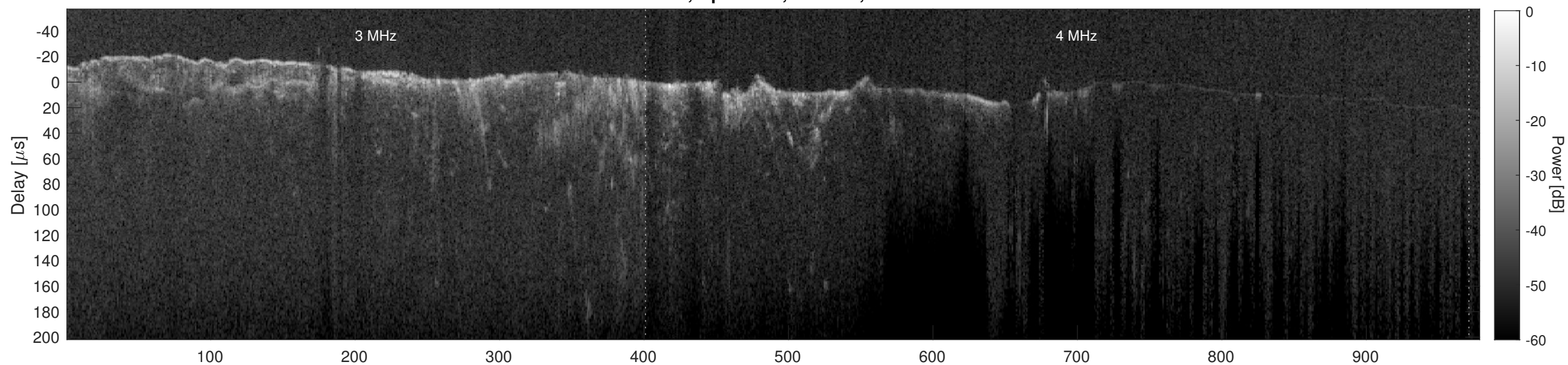
Orbit 12657, Cluttergram
