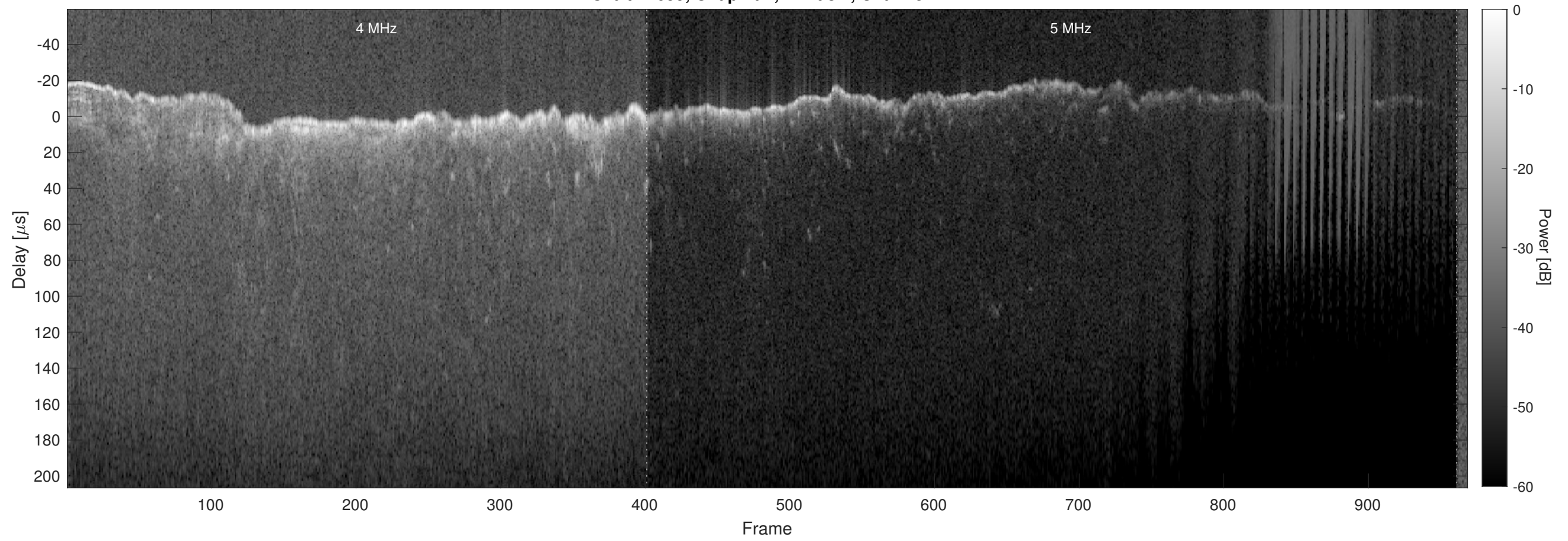
Orbit 12659, Chapman, Window, Channel 2
