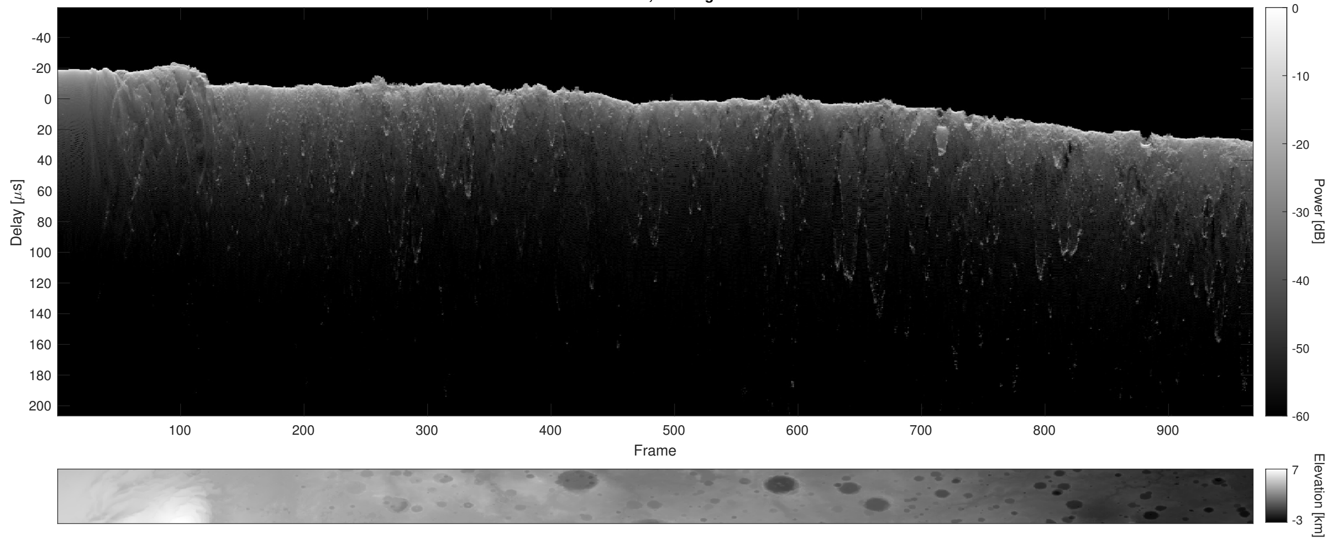
Orbit 12659, Cluttergram
