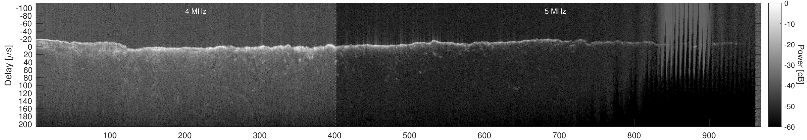
Orbit 12659, Window, Channel 1, Optimized
