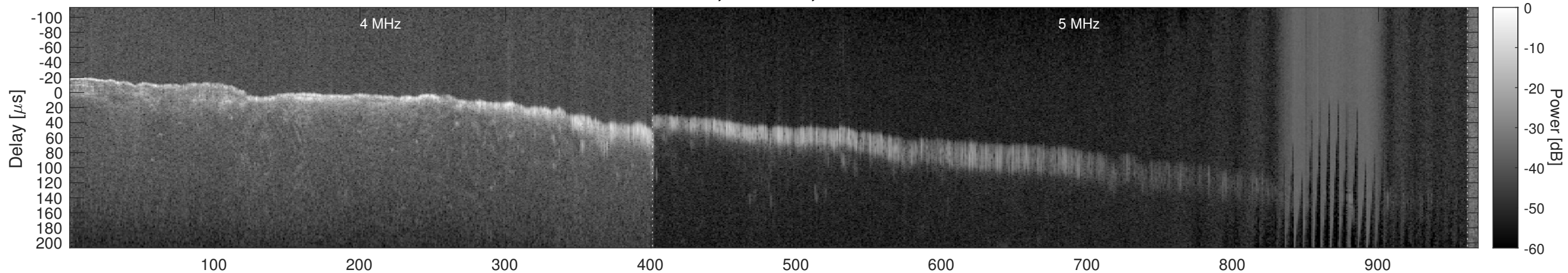
Orbit 12659, Window, Channel 1, Chapman
