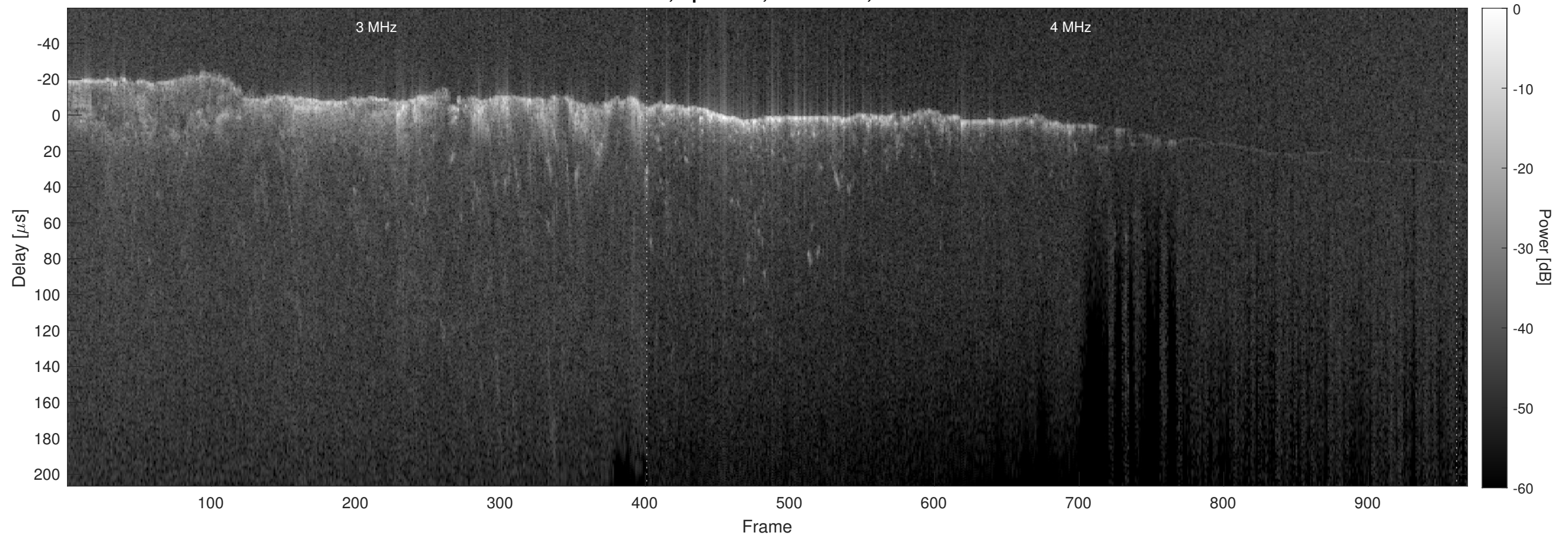
Orbit 12659, Optimized, No Window, Channel 2
