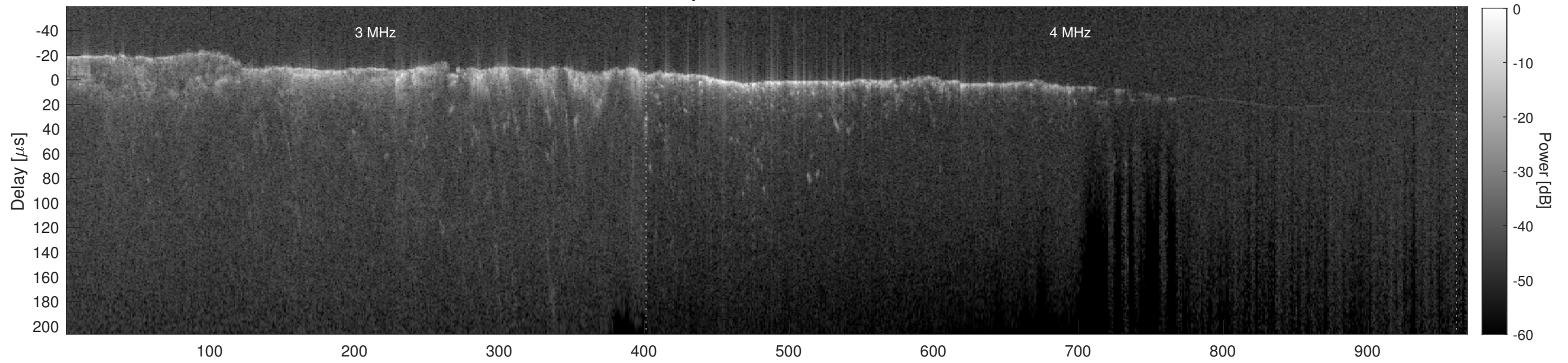
Orbit 12659, Cluttergram
