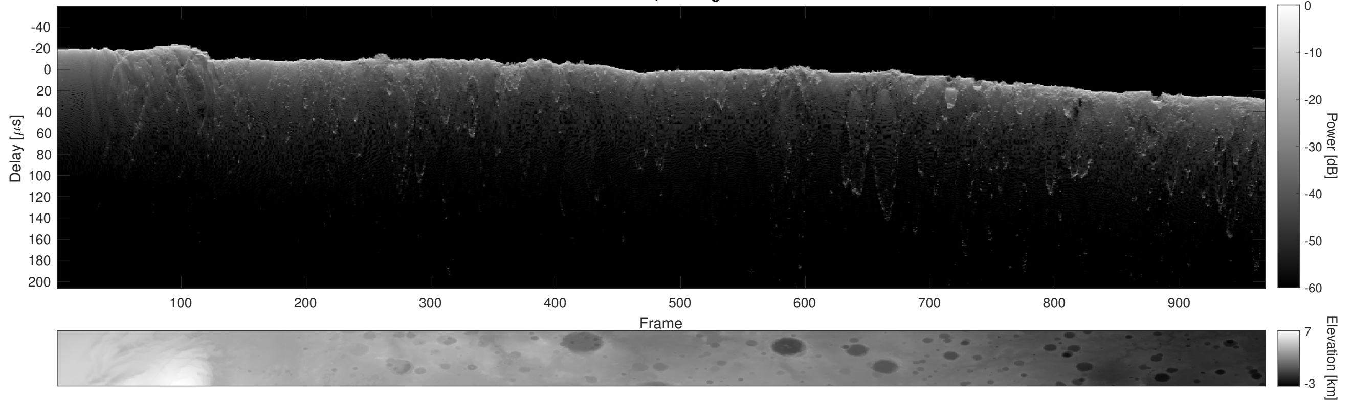
Orbit 12659, Cluttergram
