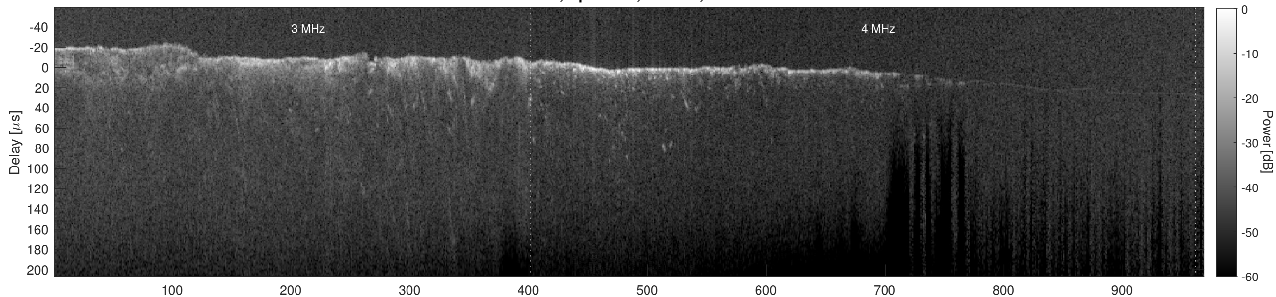
Orbit 12659, Cluttergram
