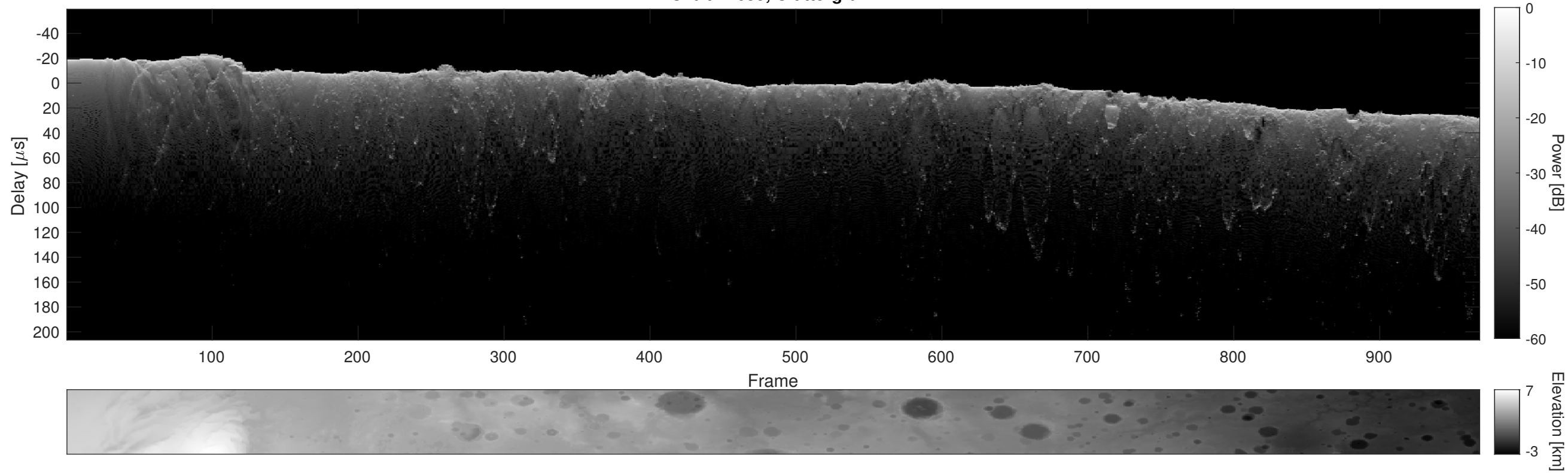
Orbit 12659, Cluttergram
