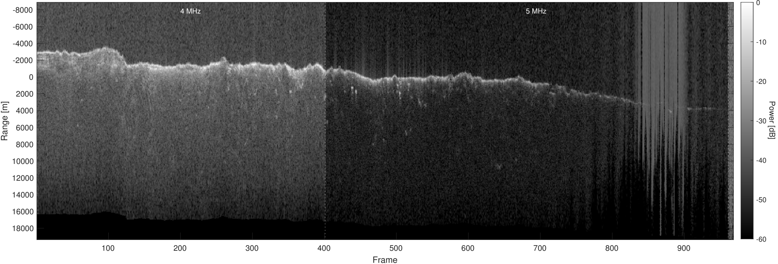
Orbit 12659, Optimized, Window, Depth-Corrected, Channel 2
