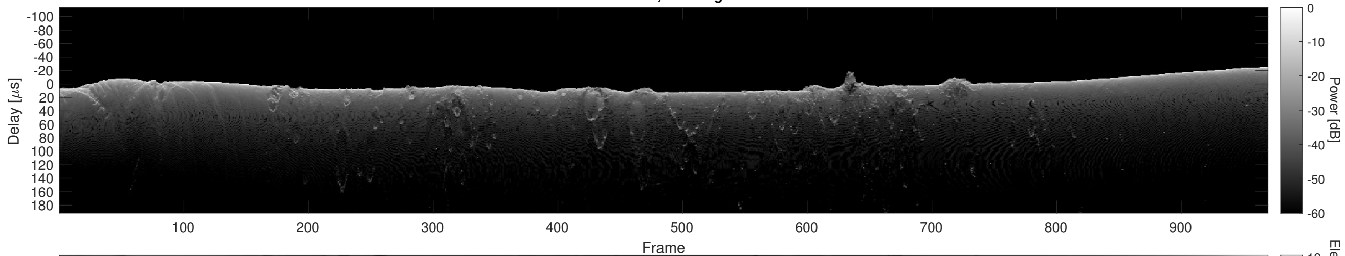
Orbit 12660, Cluttergram
