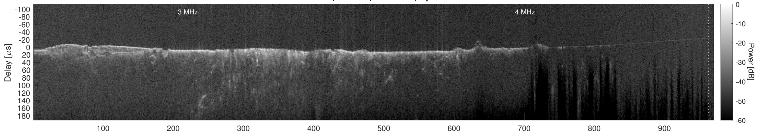
Orbit 12660, Cluttergram
