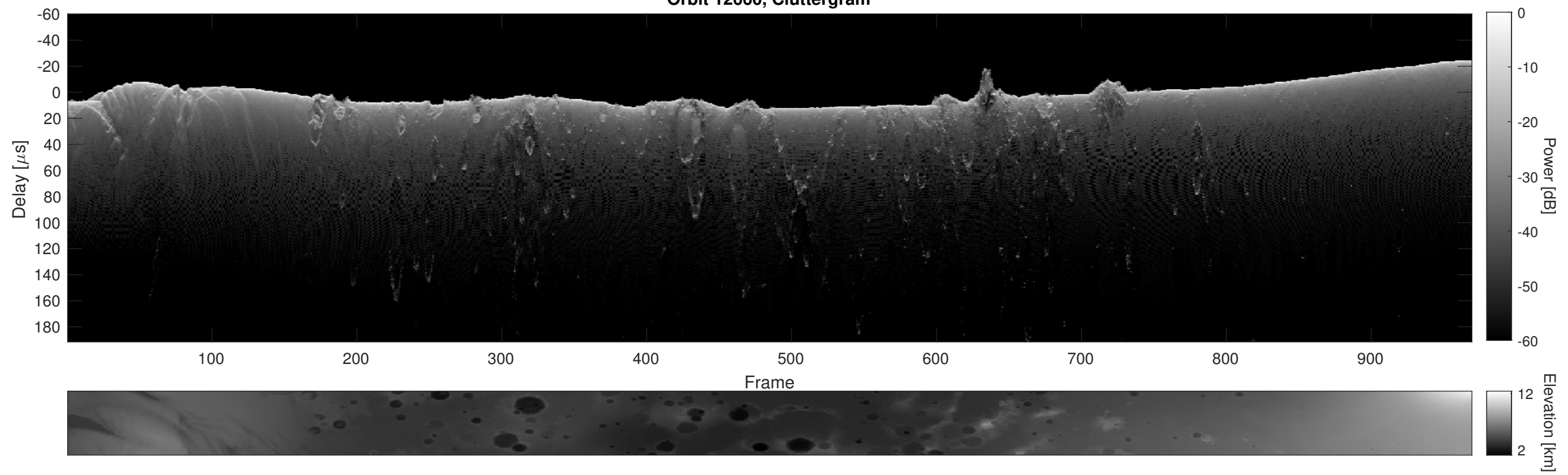
Orbit 12660, Cluttergram
