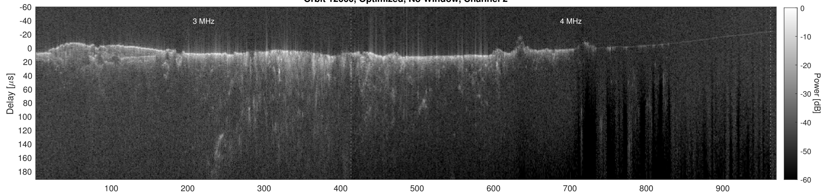
Orbit 12660, Cluttergram
