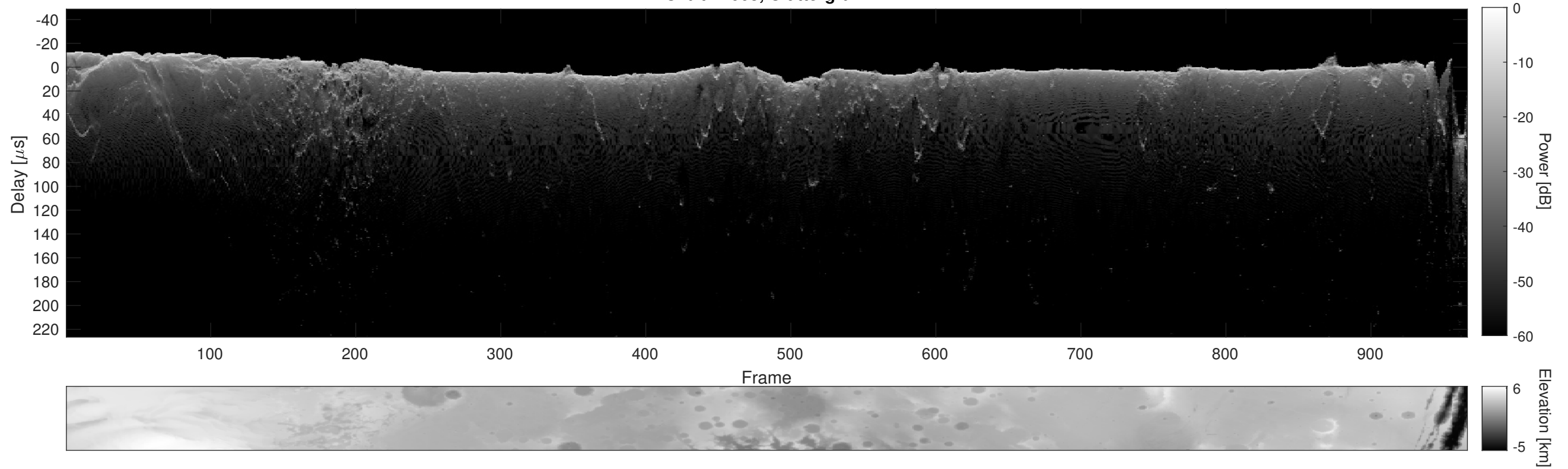
Orbit 12663, Cluttergram
