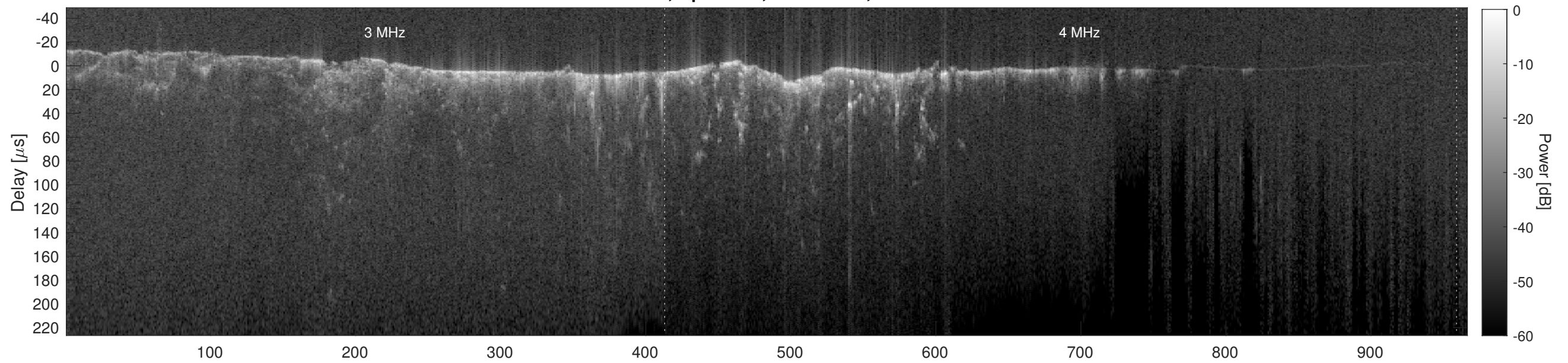
Orbit 12663, Cluttergram
