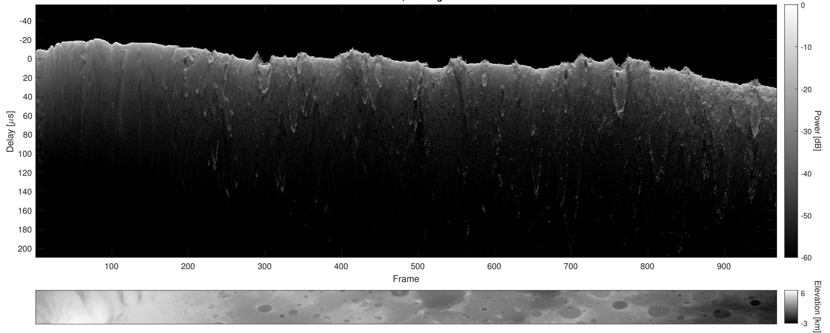
Orbit 12664, Cluttergram
