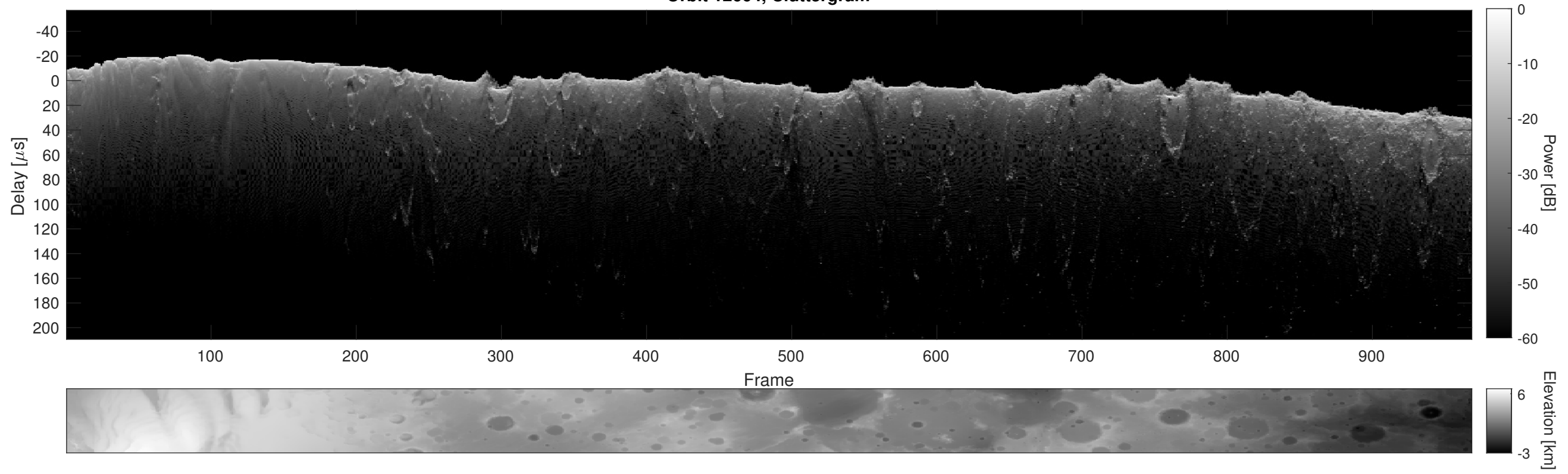
Orbit 12664, Cluttergram
