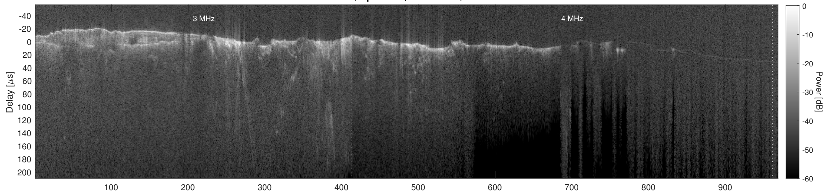
Orbit 12664, Cluttergram
