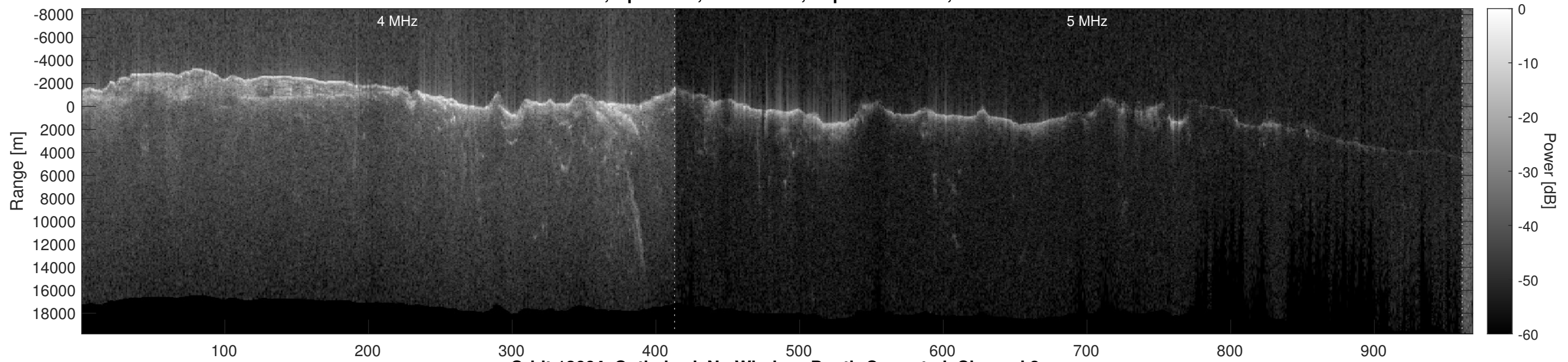
Orbit 12664, Optimized, No Window, Depth-Corrected, Channel 2
