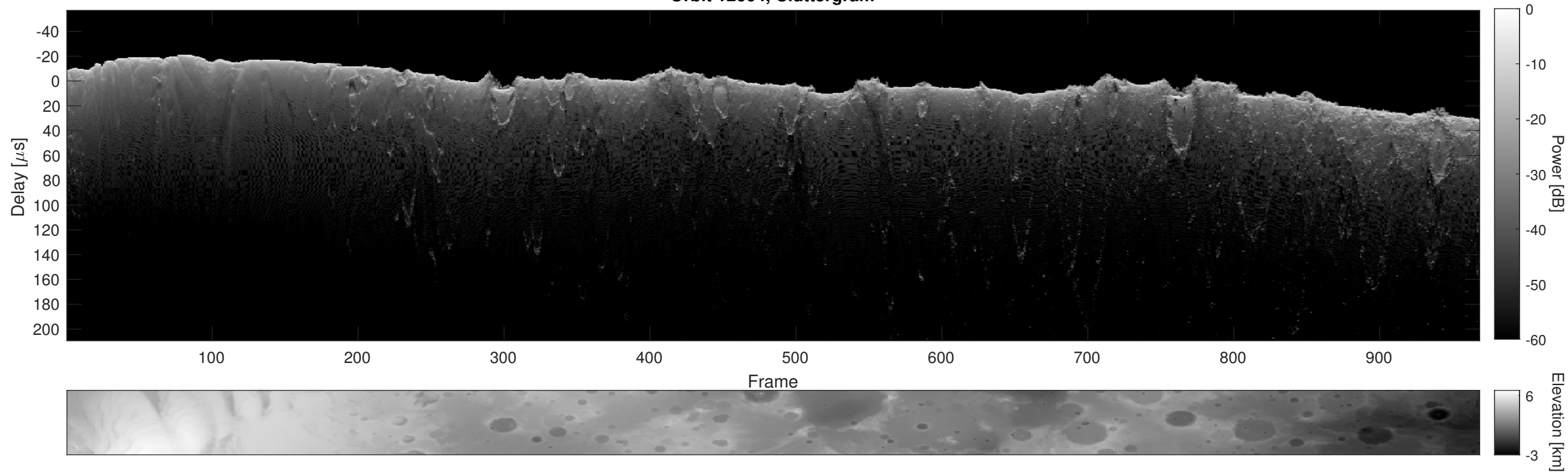
Orbit 12664, Cluttergram
