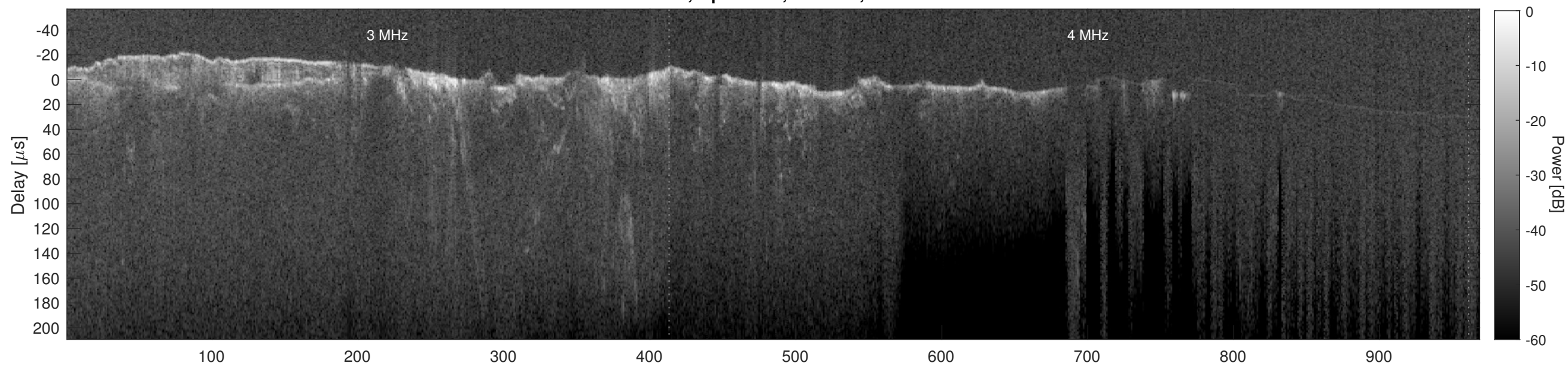
Orbit 12664, Cluttergram
