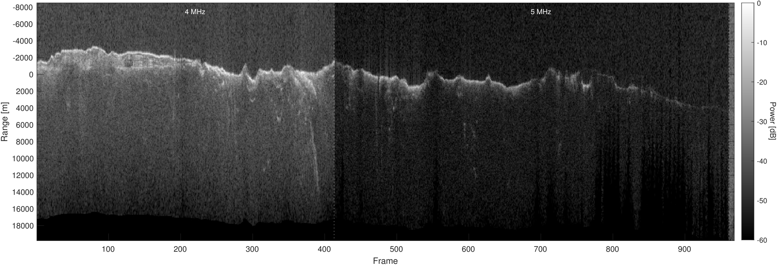
Orbit 12664, Optimized, Window, Depth-Corrected, Channel 2
