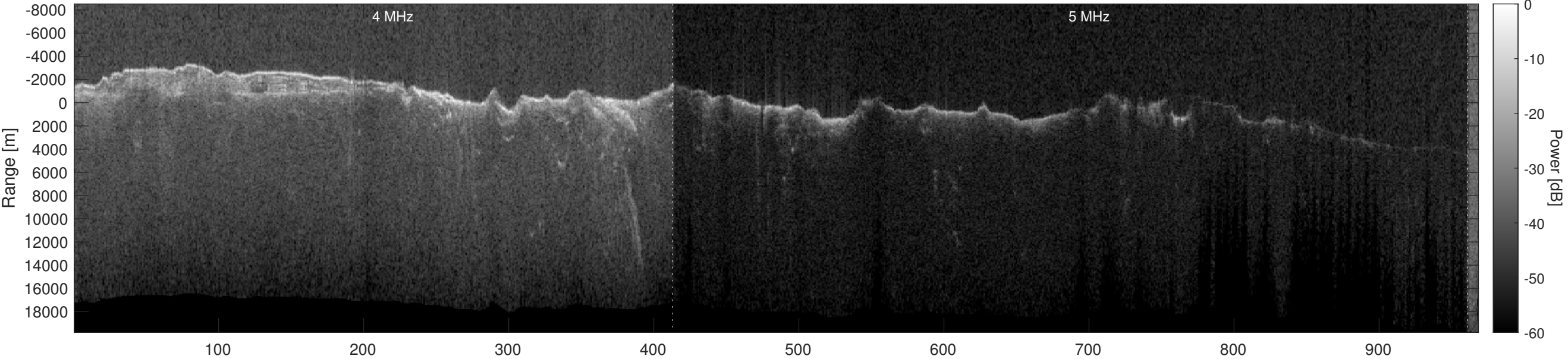
Orbit 12664, Optimized, Window, Depth-Corrected, Channel 2
