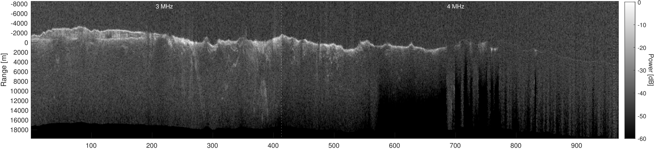
Orbit 12664, Depth-Corrected Cluttergram
