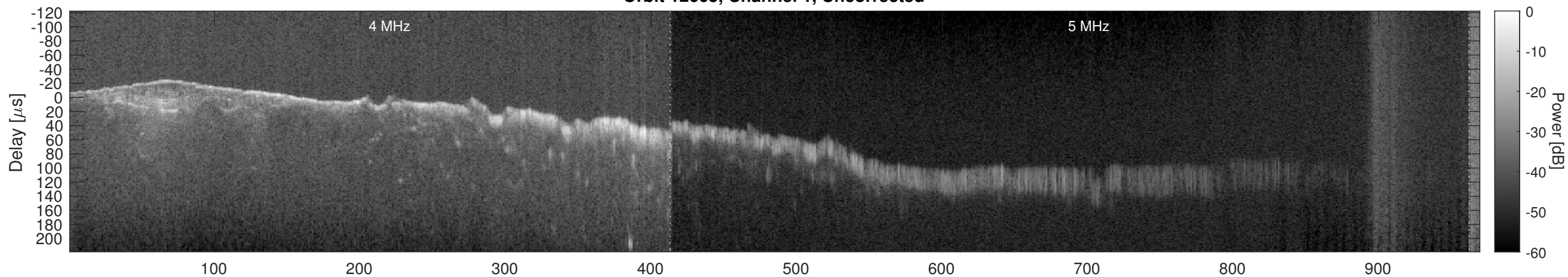
Orbit 12665, Window, Channel 1, Chapman
