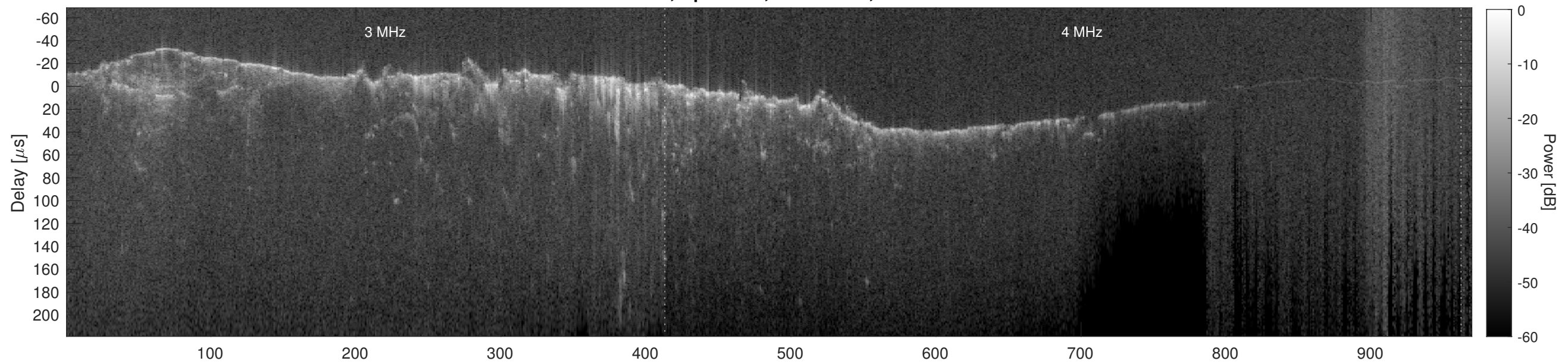
Orbit 12665, Cluttergram
