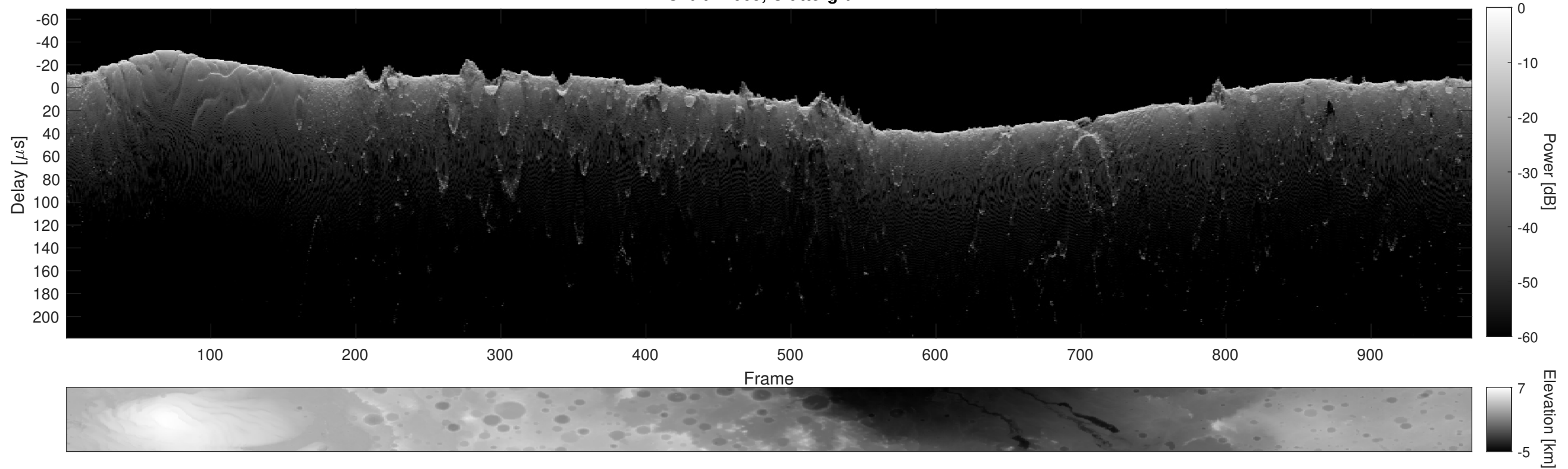
Orbit 12665, Cluttergram
