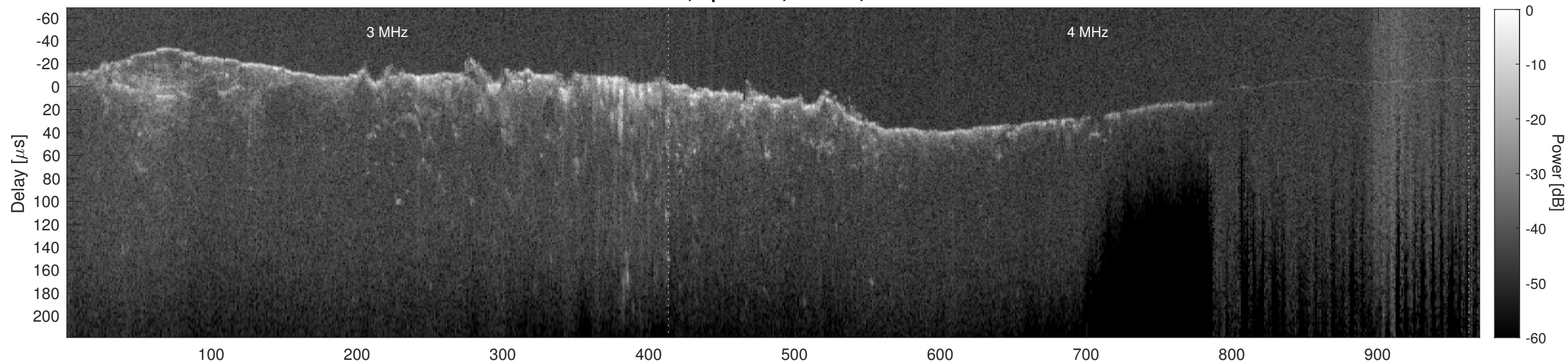
Orbit 12665, Cluttergram
