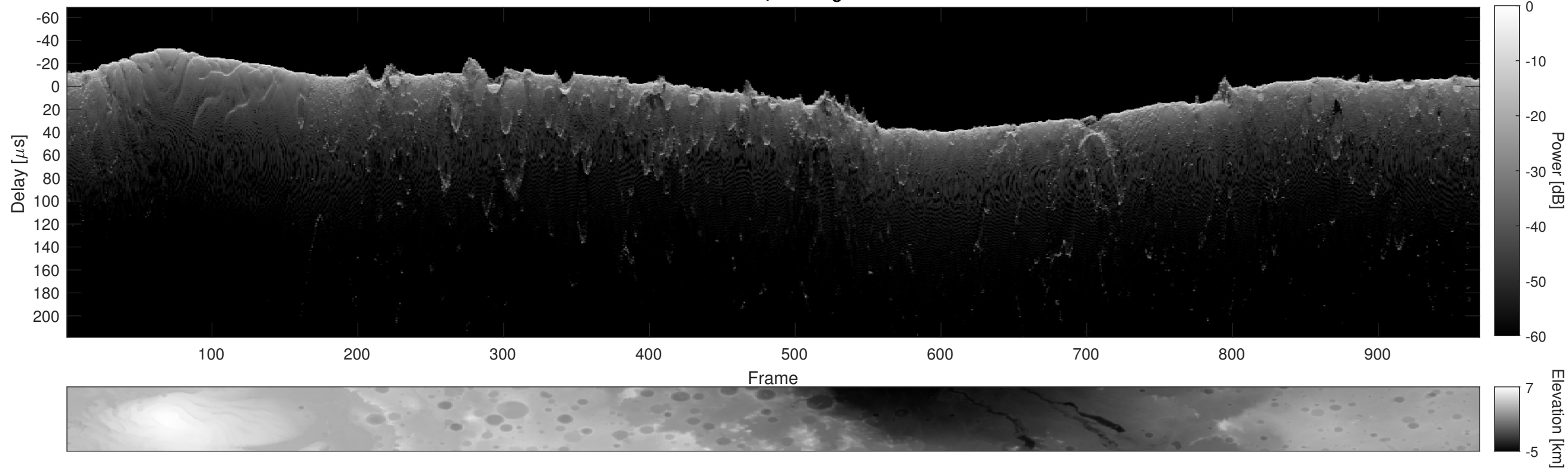
Orbit 12665, Cluttergram
