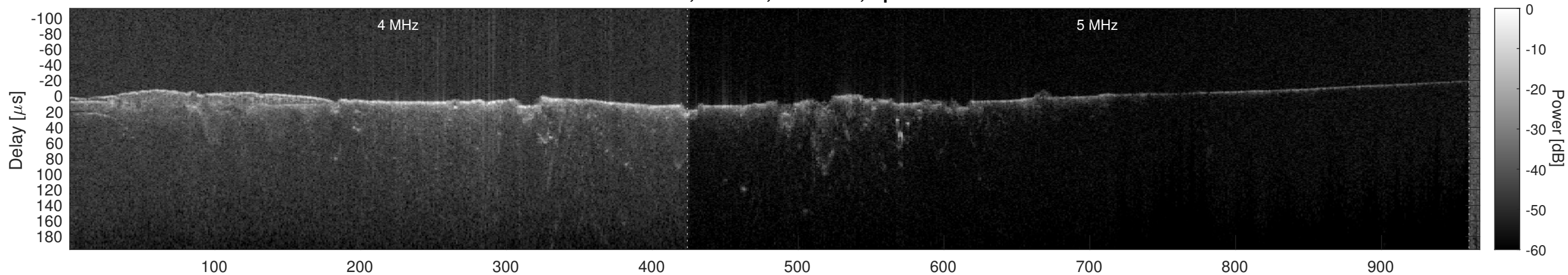
Orbit 12667, Cluttergram
