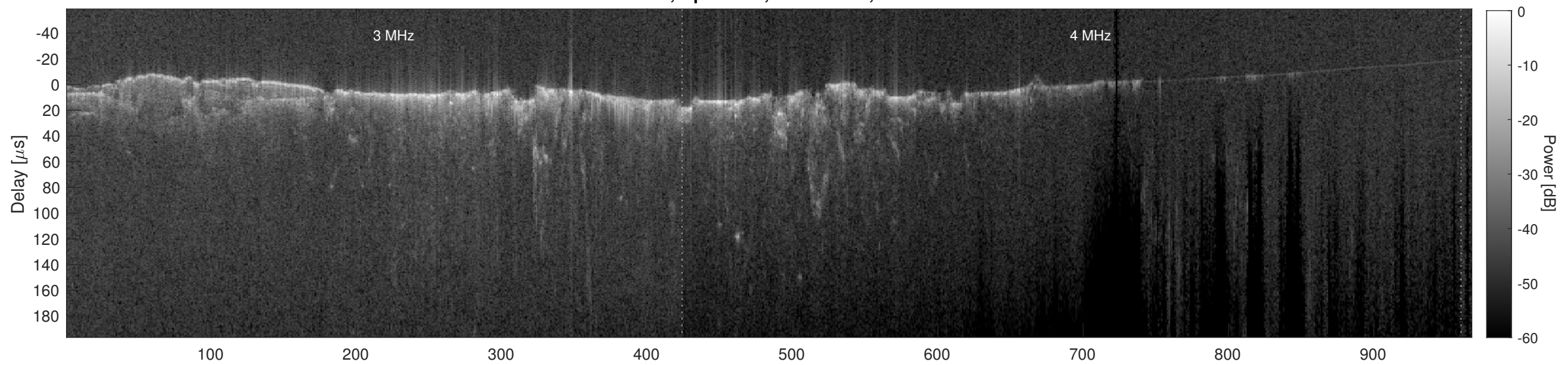
Orbit 12667, Cluttergram
