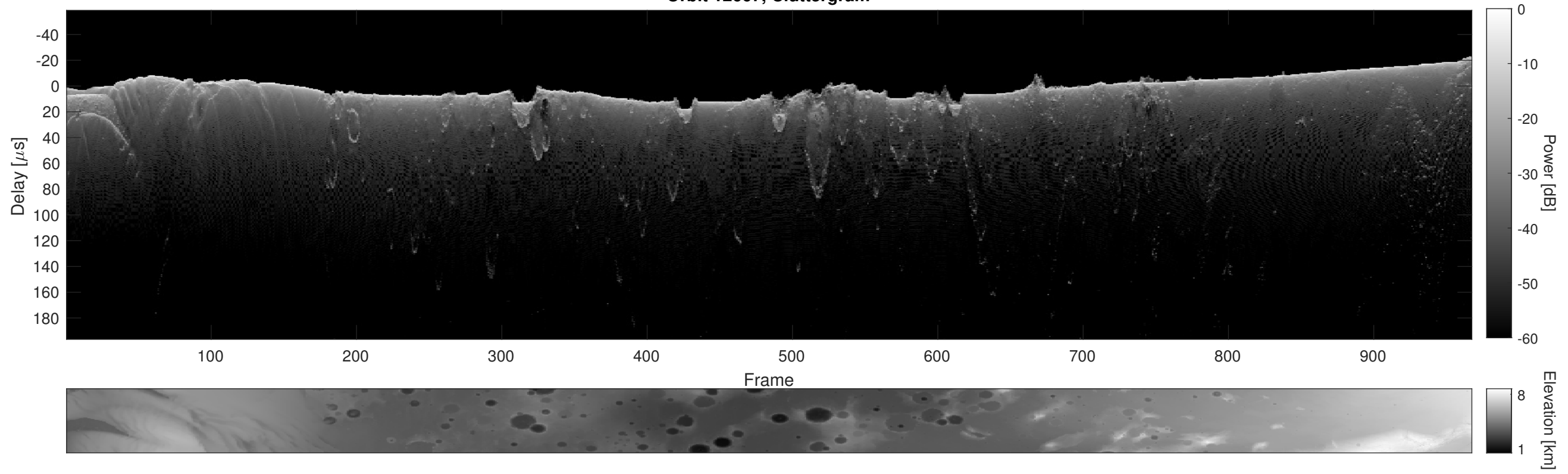
Orbit 12667, Cluttergram
