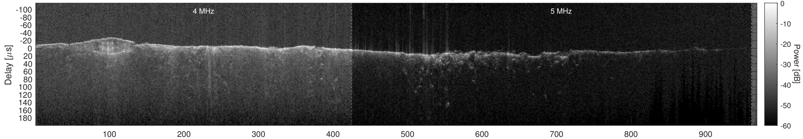
Orbit 12669, Cluttergram
