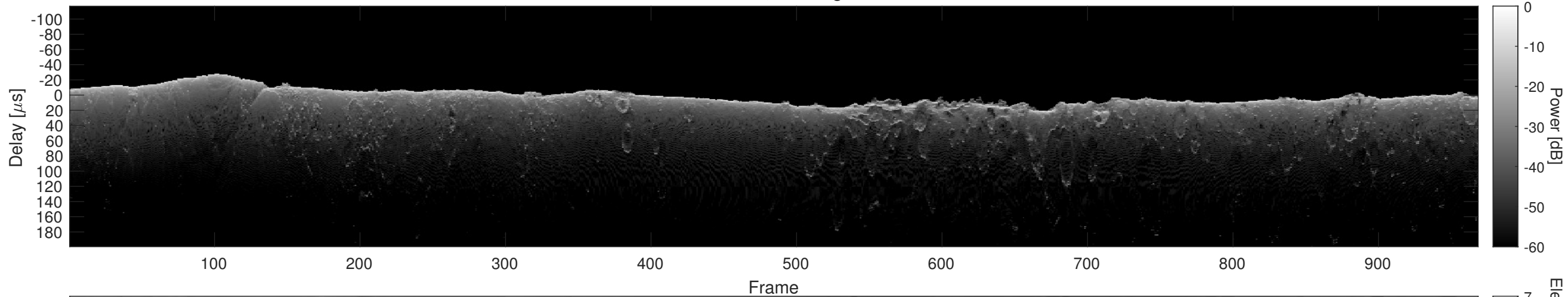
Orbit 12669, Cluttergram
