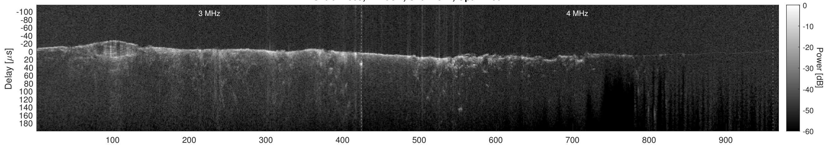
Orbit 12669, Cluttergram
