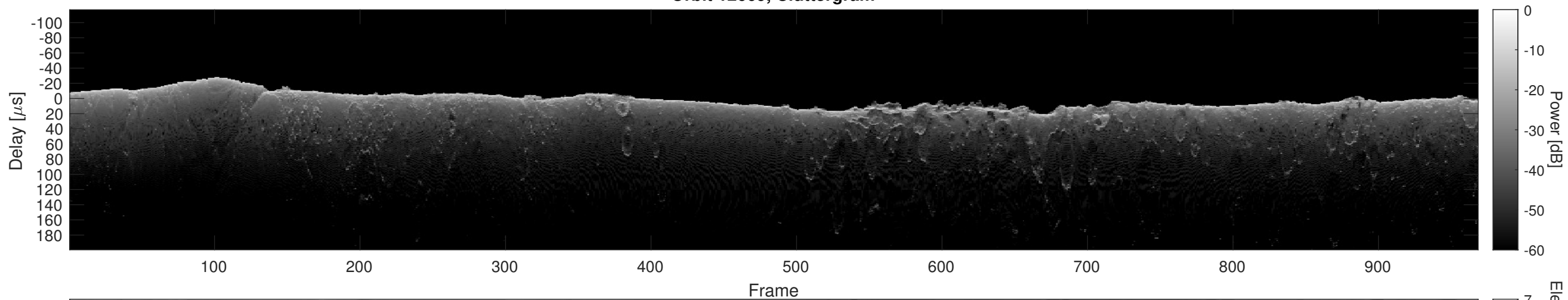
Orbit 12669, Cluttergram
