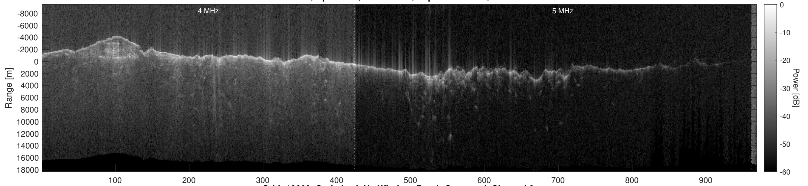
Orbit 12669, Optimized, No Window, Depth-Corrected, Channel 2
