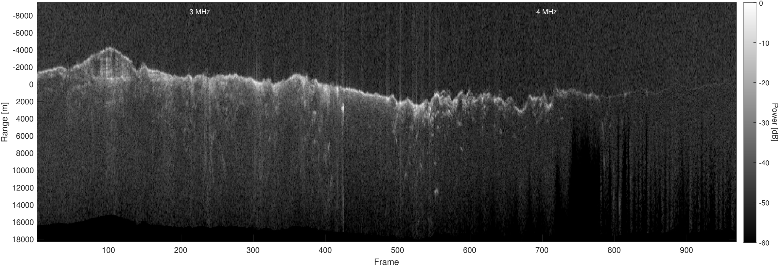
Orbit 12669, Optimized, Window, Depth-Corrected, Channel 2
