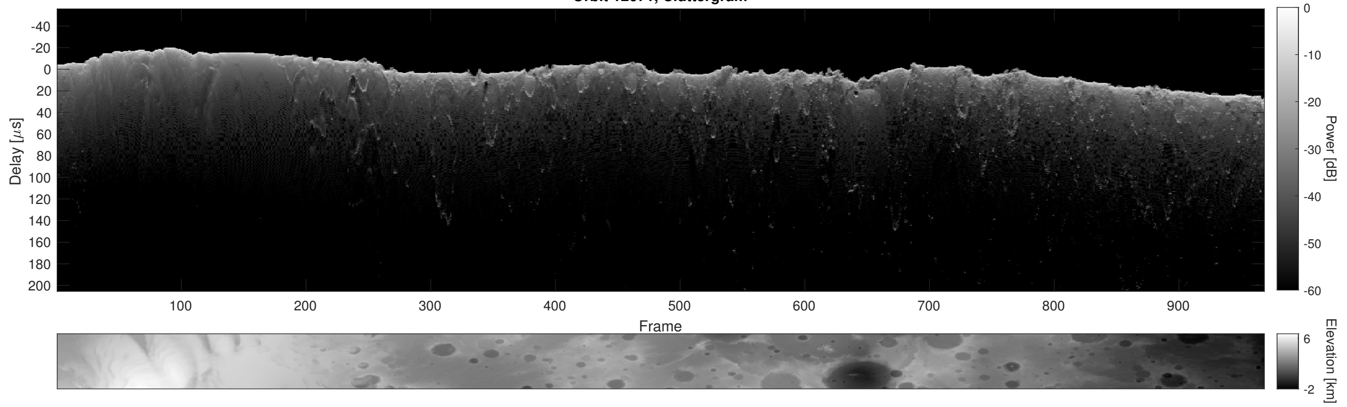
Orbit 12671, Cluttergram
