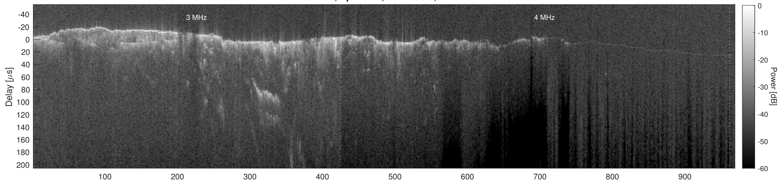
Orbit 12671, Cluttergram
