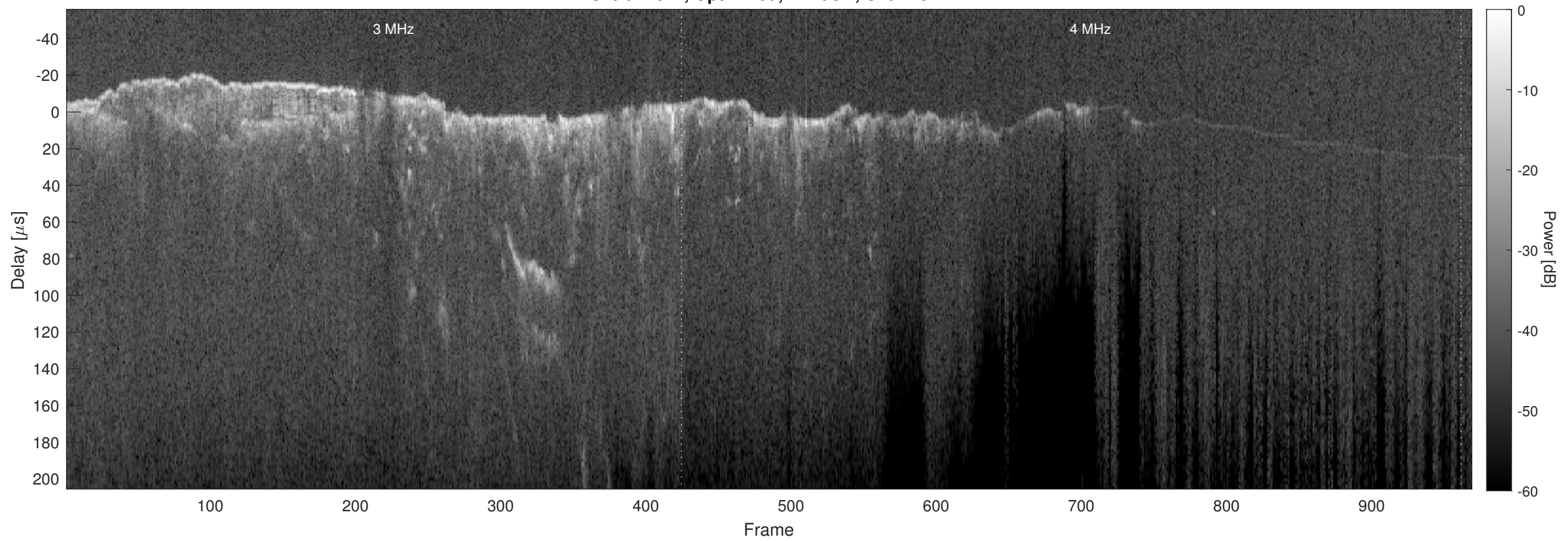
Orbit 12671, Optimized, Window, Channel 2
