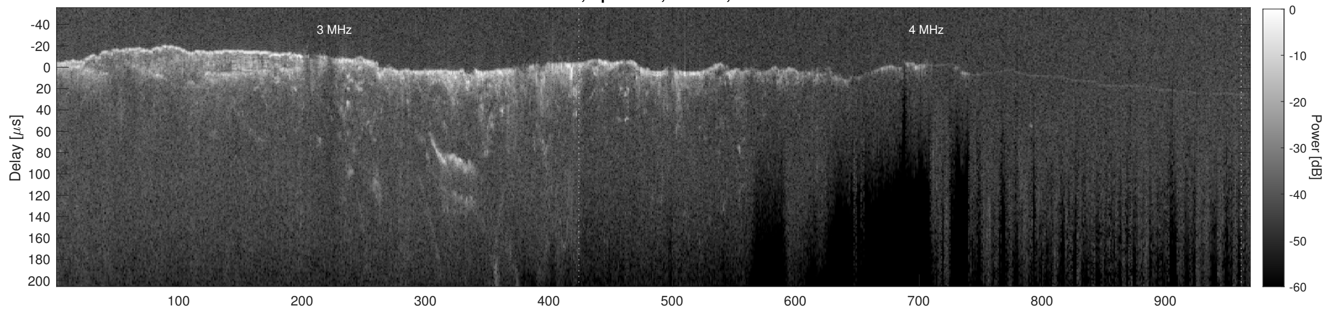
Orbit 12671, Cluttergram
