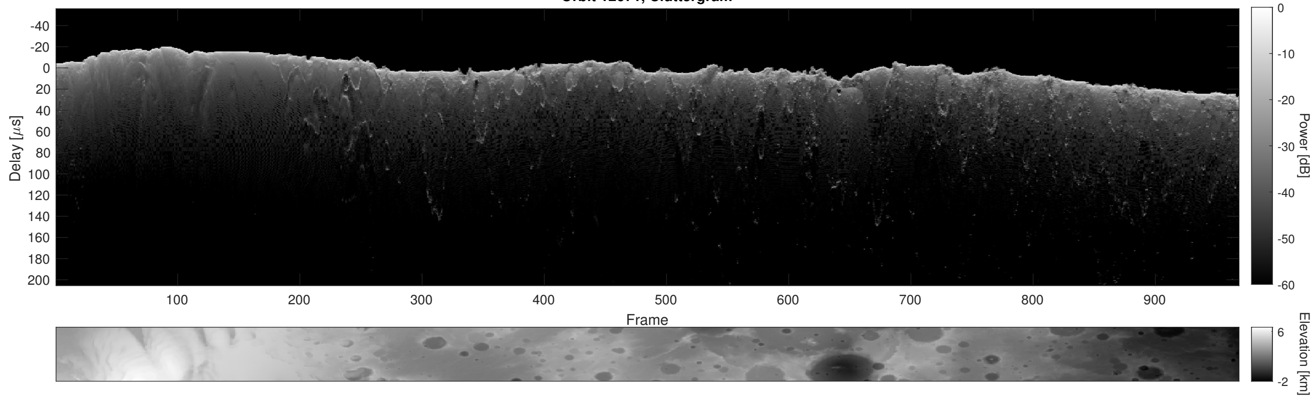
Orbit 12671, Cluttergram
