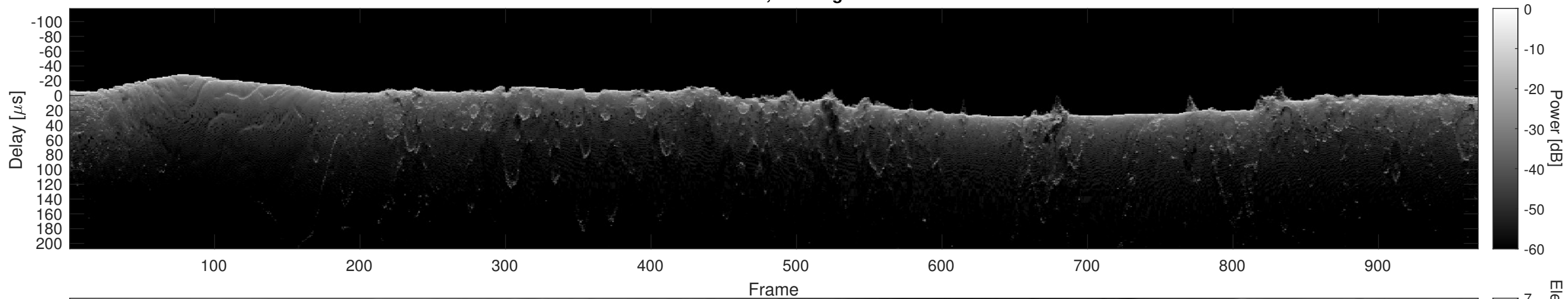
Orbit 12672, Cluttergram
